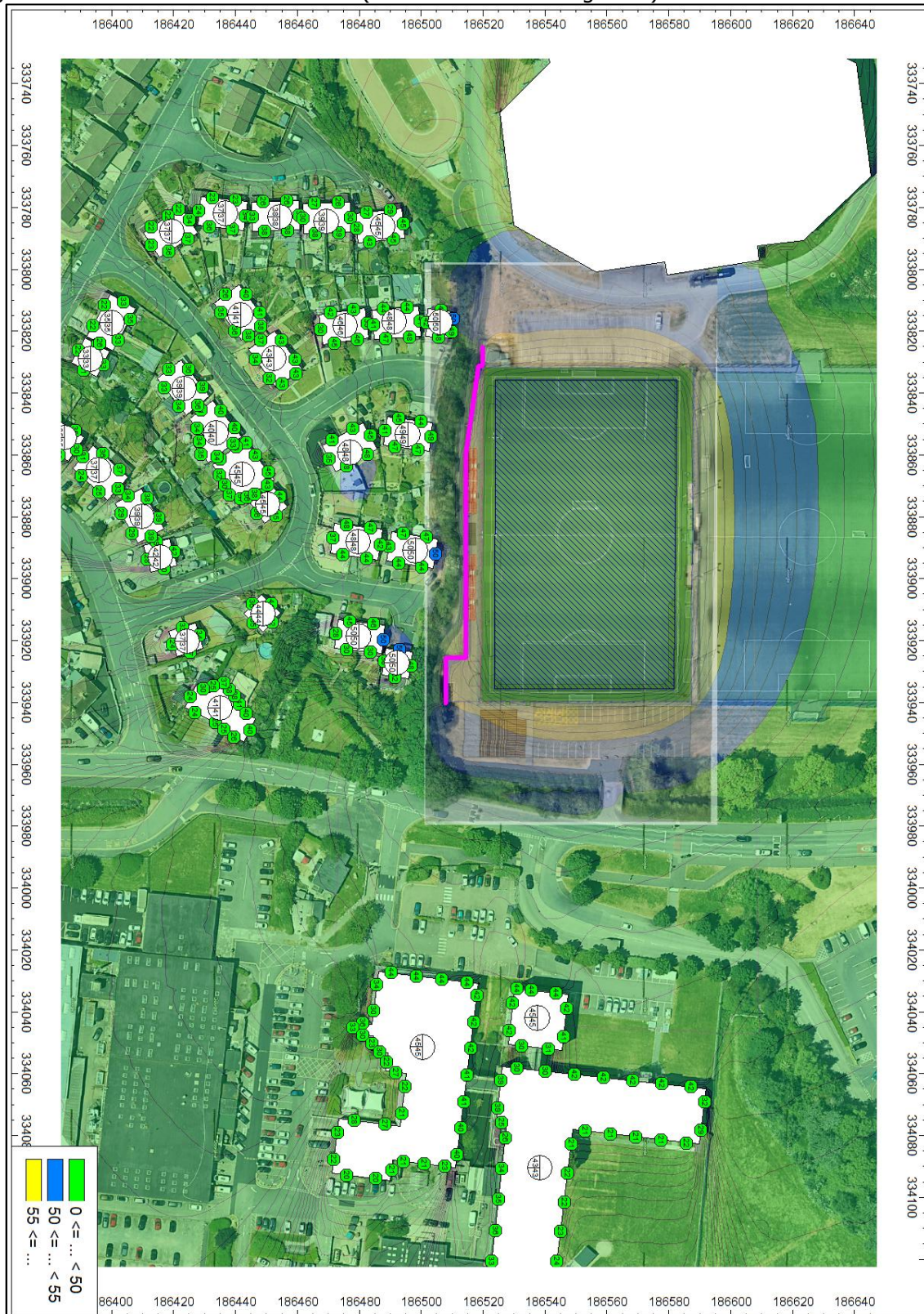
Figure 9: Predicted AGP Noise Emission (1.5 metres above the ground).
