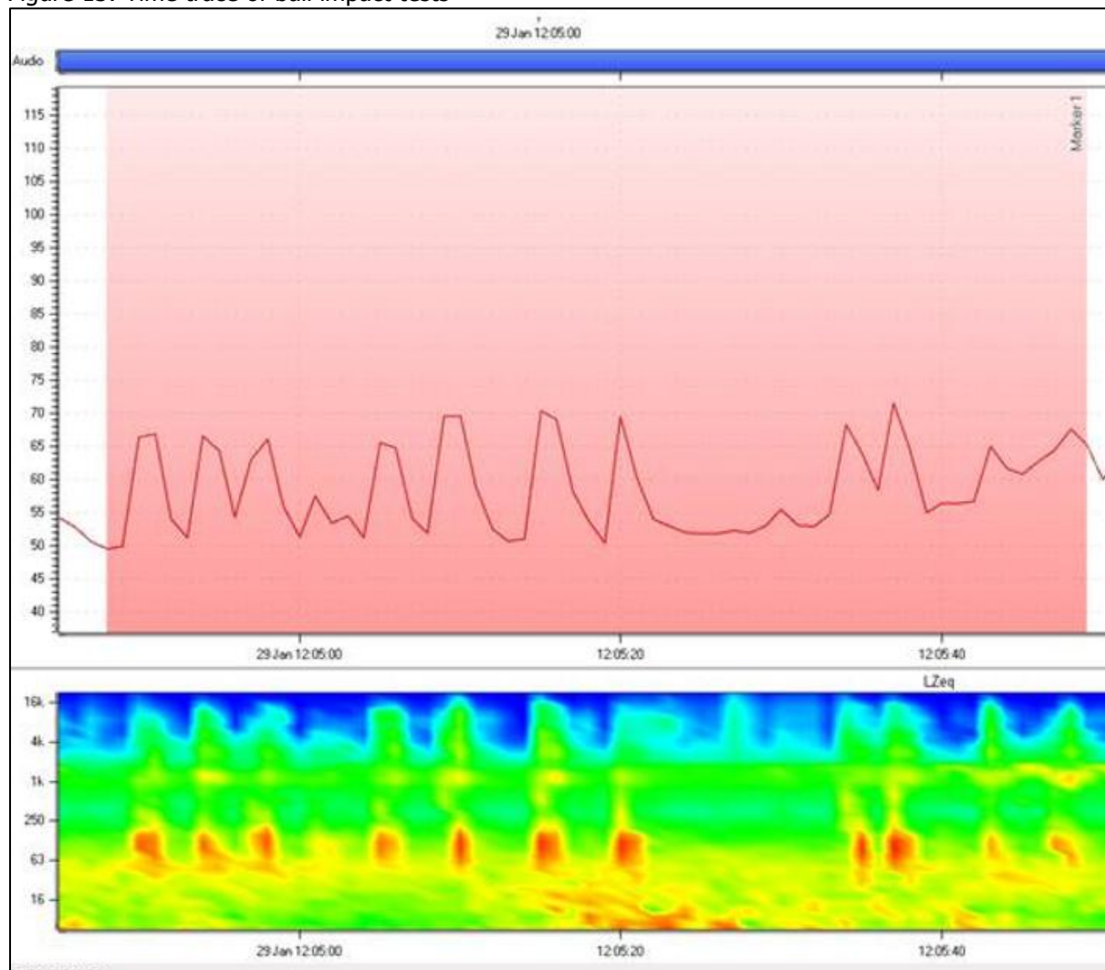
Figure 13: Time trace of ball impact tests
