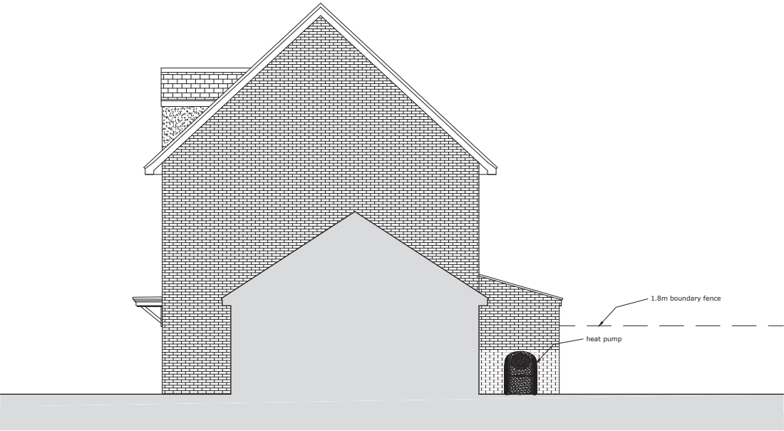
East Elevation as PROPOSED 1:50
