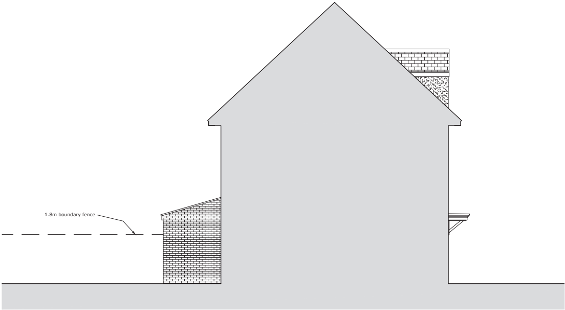
West Elevation as PROPOSED 1:50
