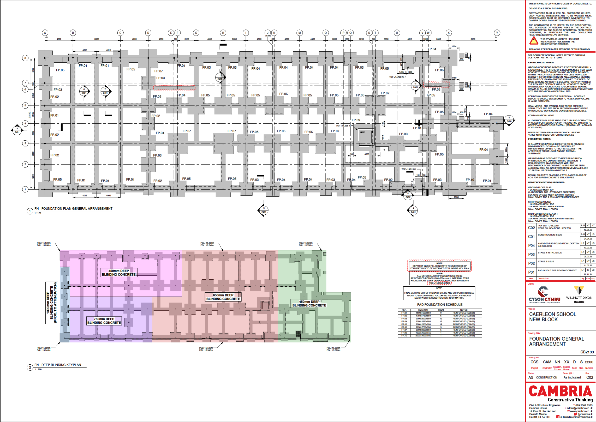
Figure 4: Plan showing layout and required depth of foundations (Provided by the client)
