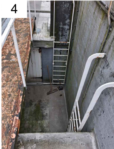
Roof well to be boarded over and new access hatch and ladder to be provided
