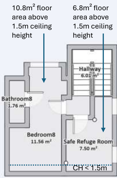
Proposed Second Floor
