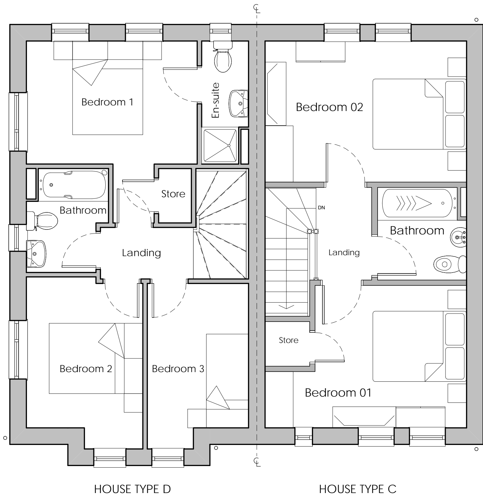
First Floor 1 : 50
