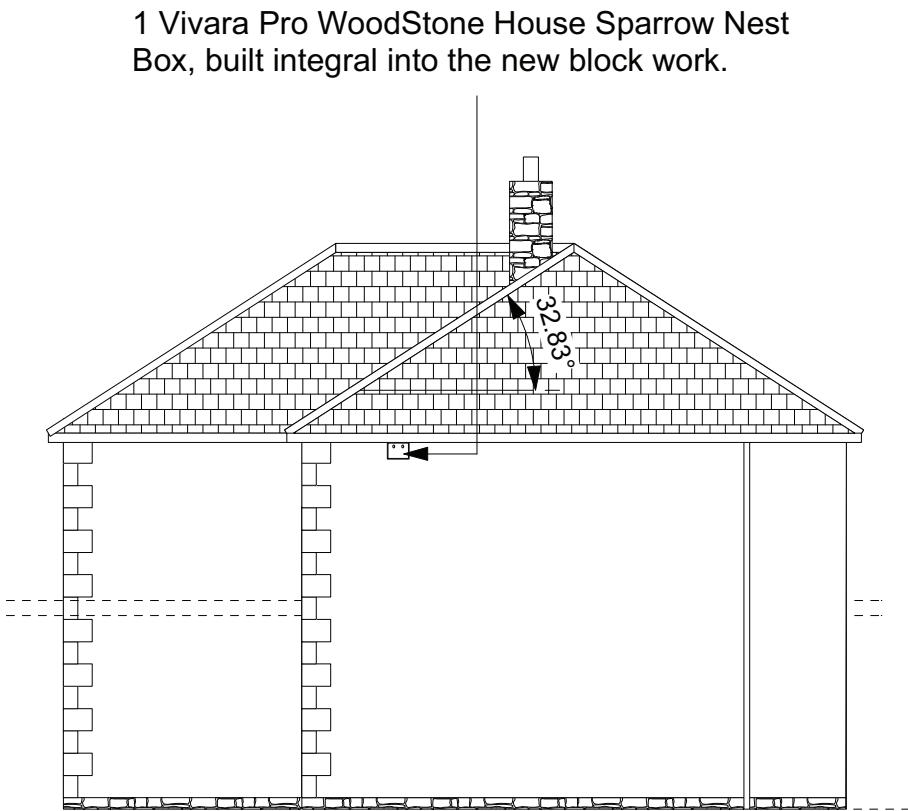
SIDE (NORTH) ELEVATION
