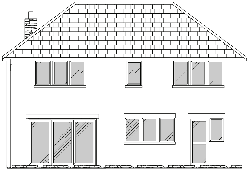
REAR (WEST) ELEVATION
