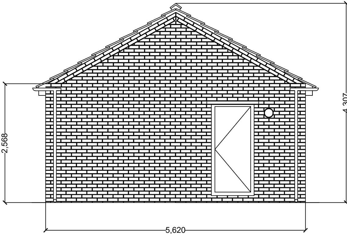
West Elevation
