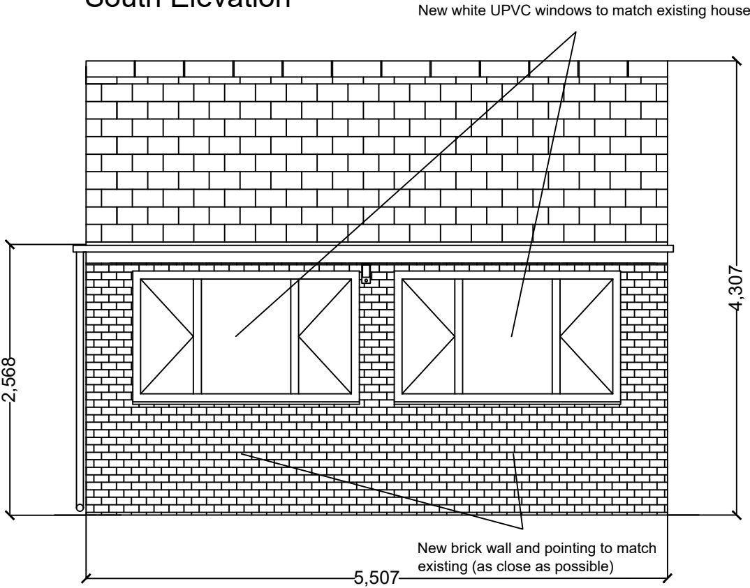
South Elevation
