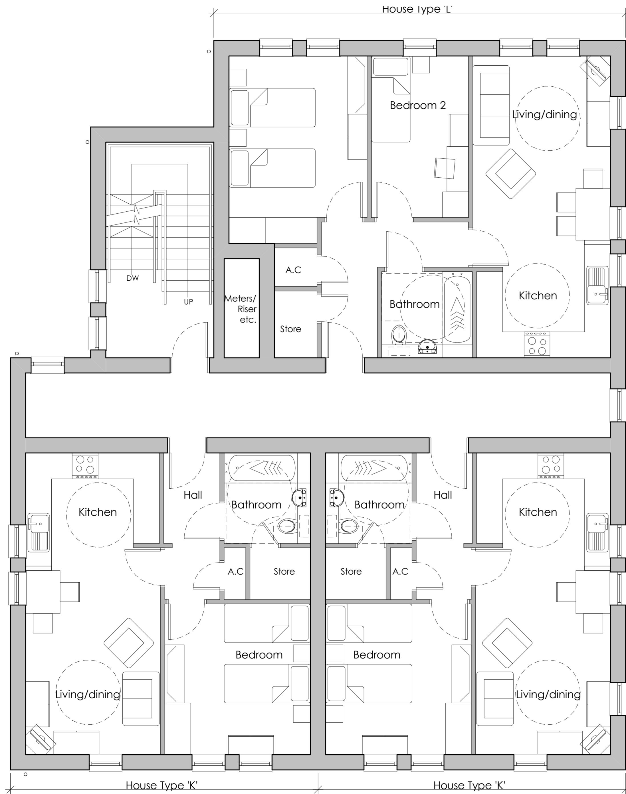
First Floor Plan House Type 'K & L'
