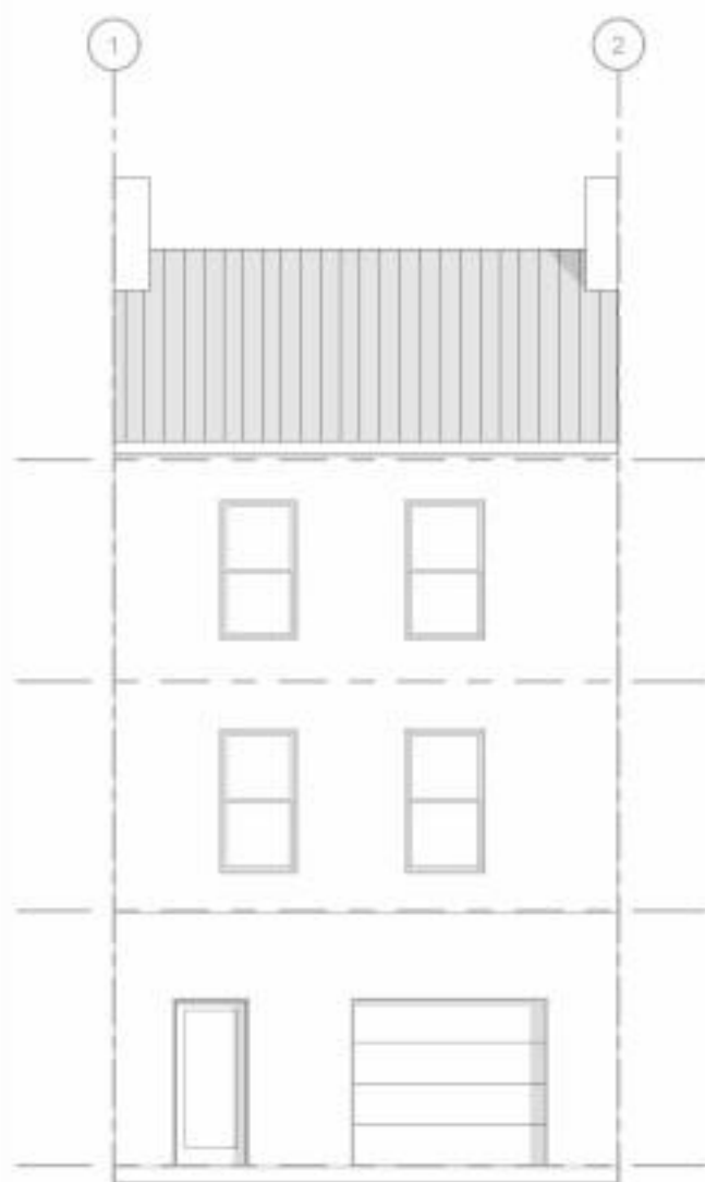
FRONT ELEVATION 1 : 50
