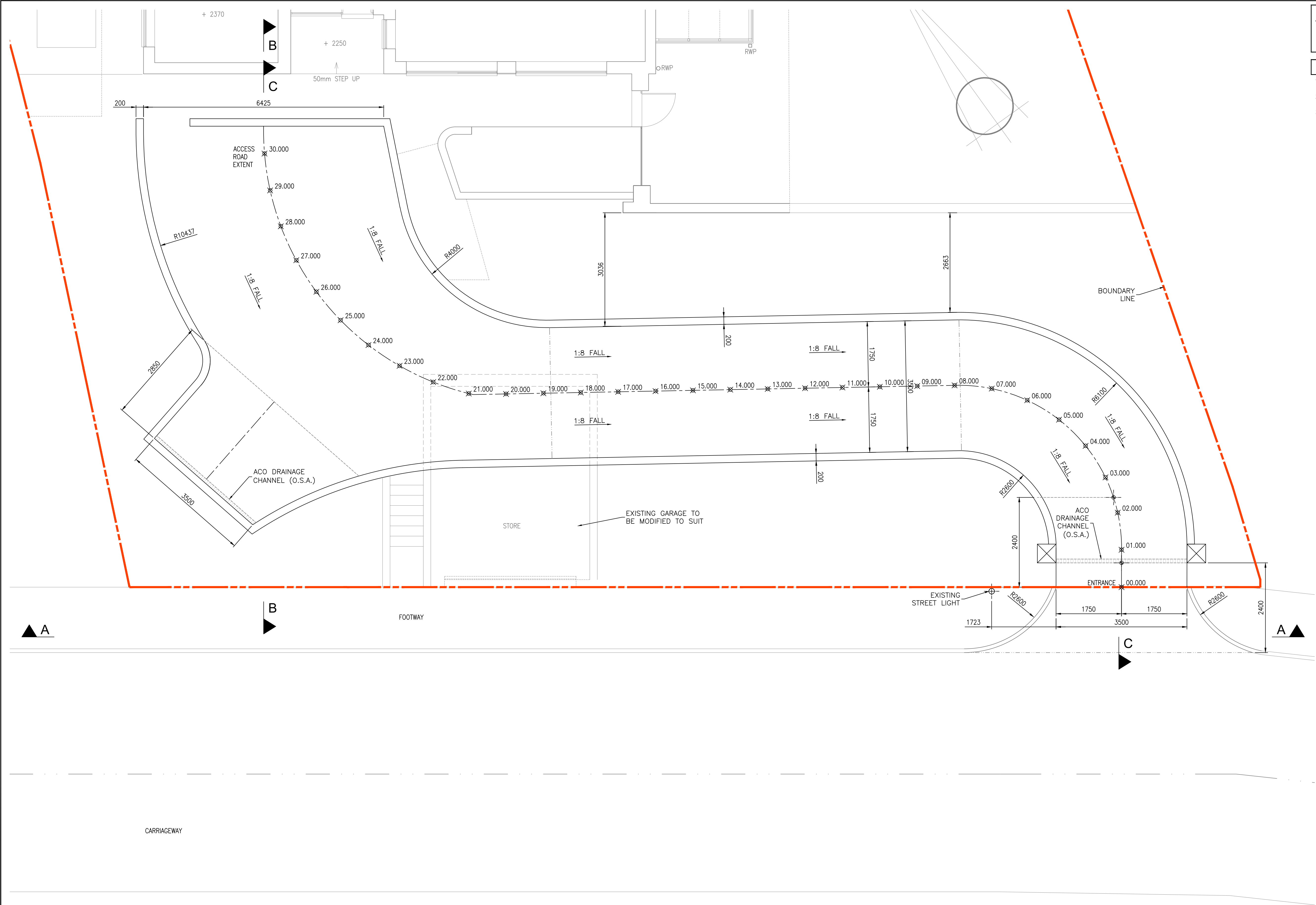
ACCESS ROAD PLAN SCALE 1:50
