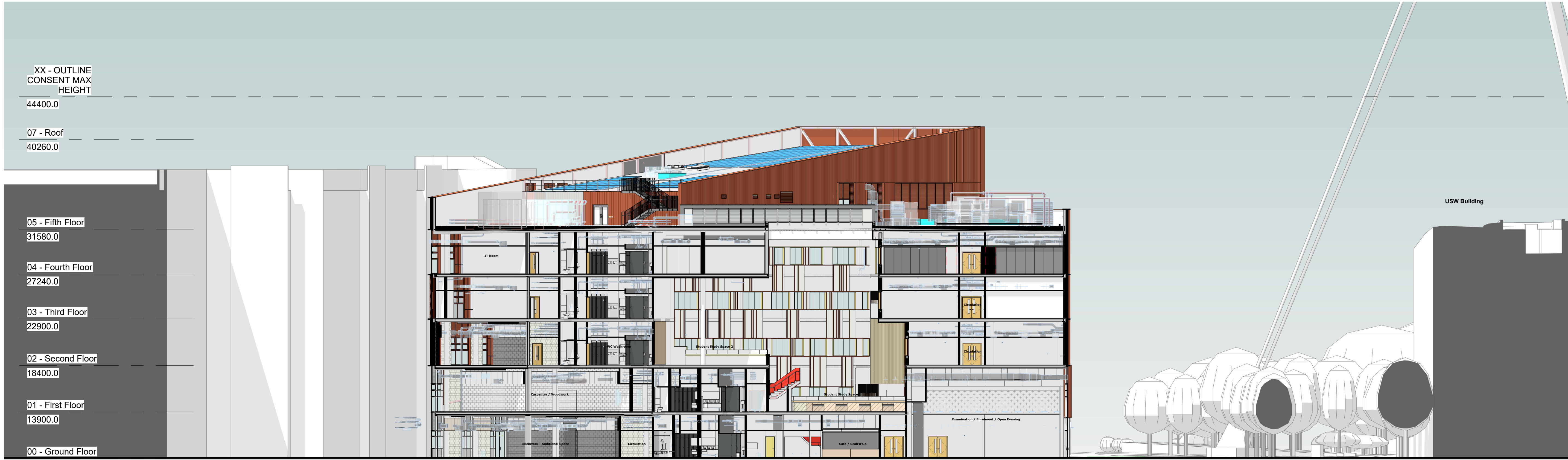
1 | Planning - GA Section Looking North 1 : 200
