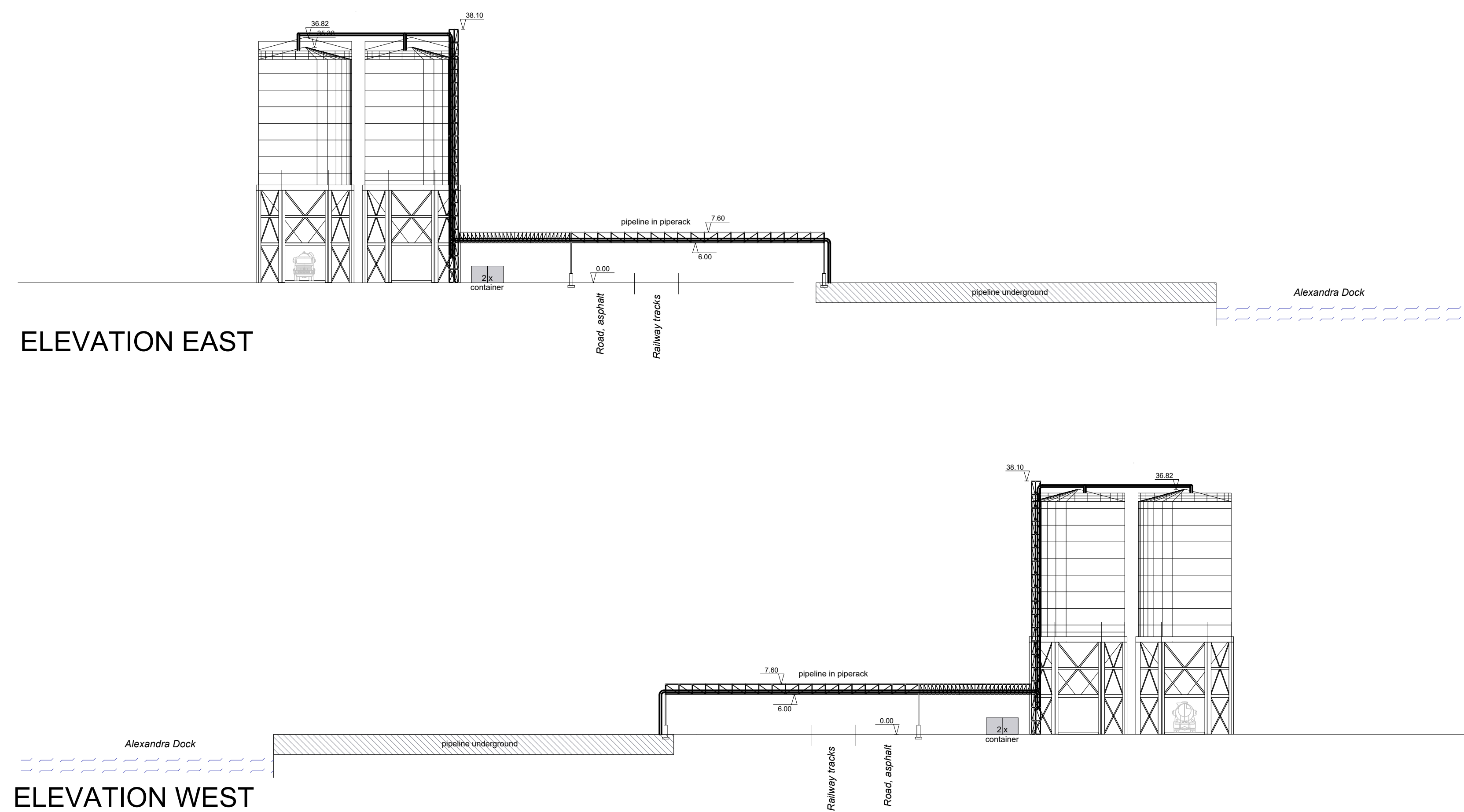
ELEVATION WEST
