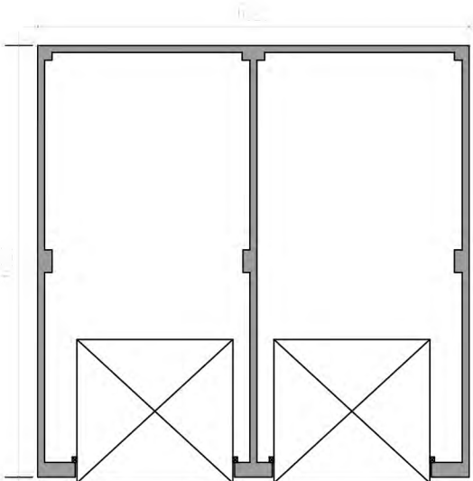
FLOOR PLAN
