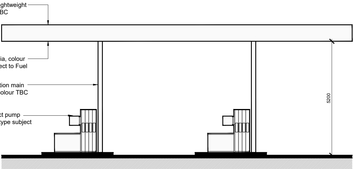
Petrol Canopy Side Elevation Scale 1:100
