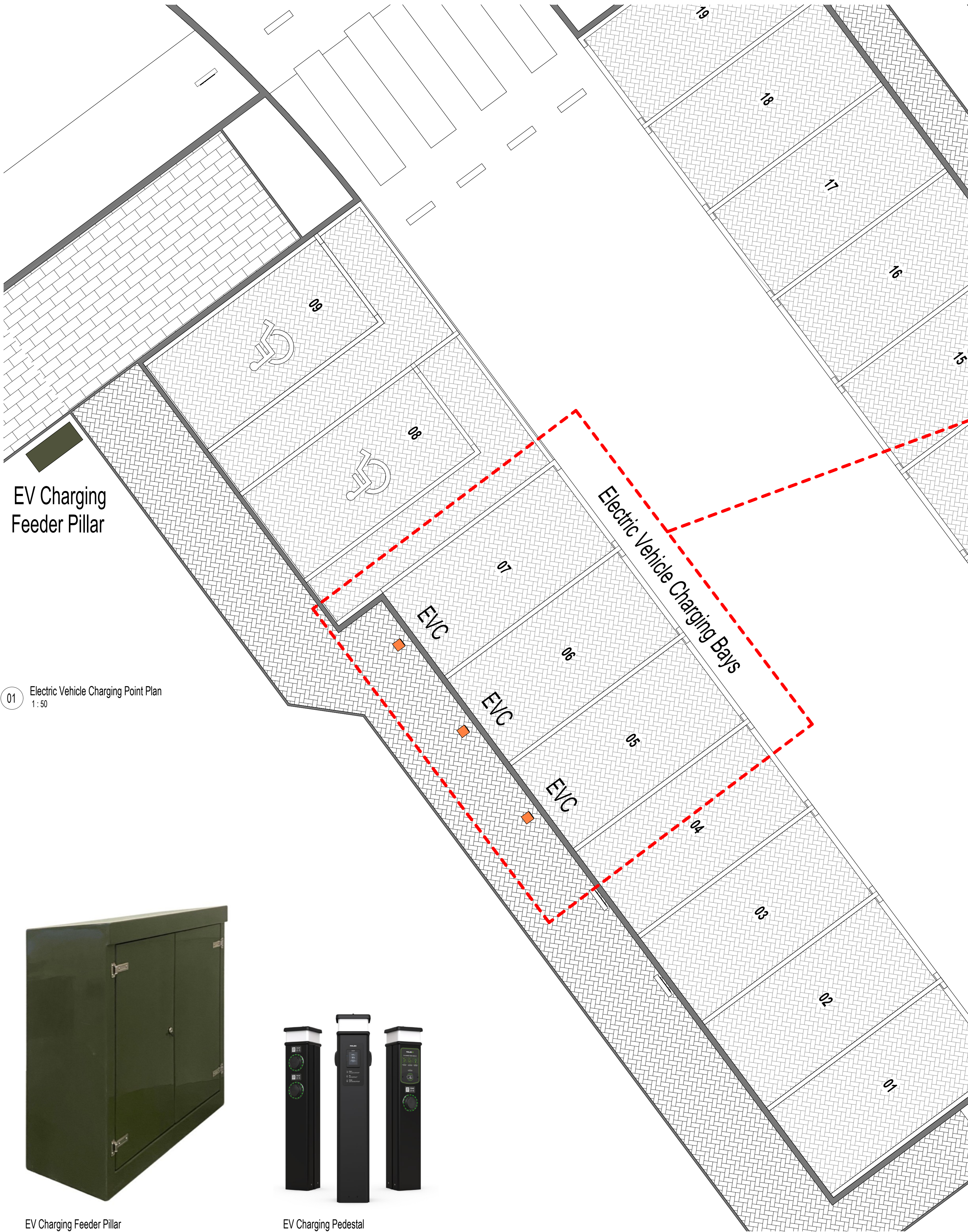
EV Charging Feeder Pillar
