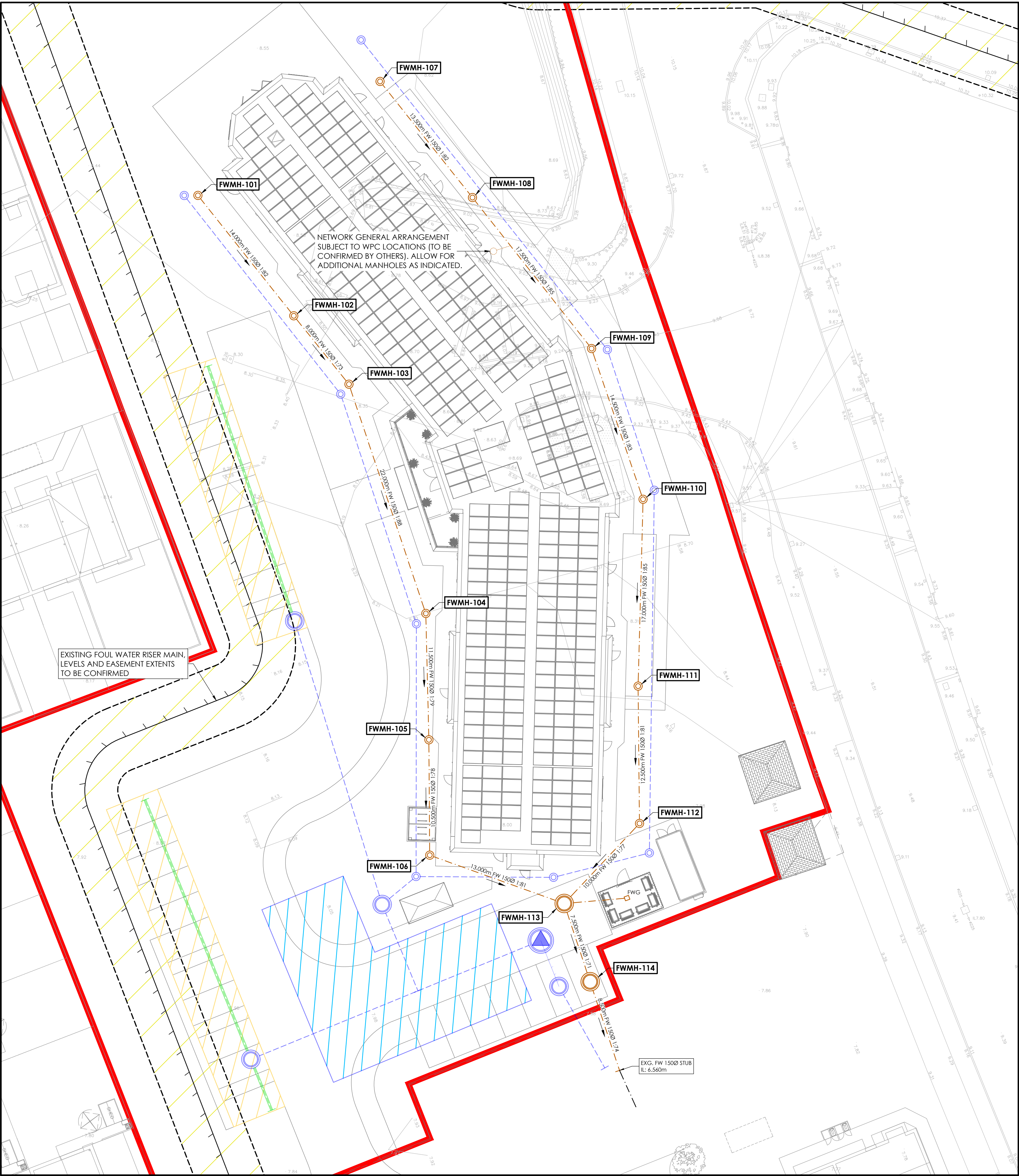
FOUL WATER DRAINAGE STRATEGY
