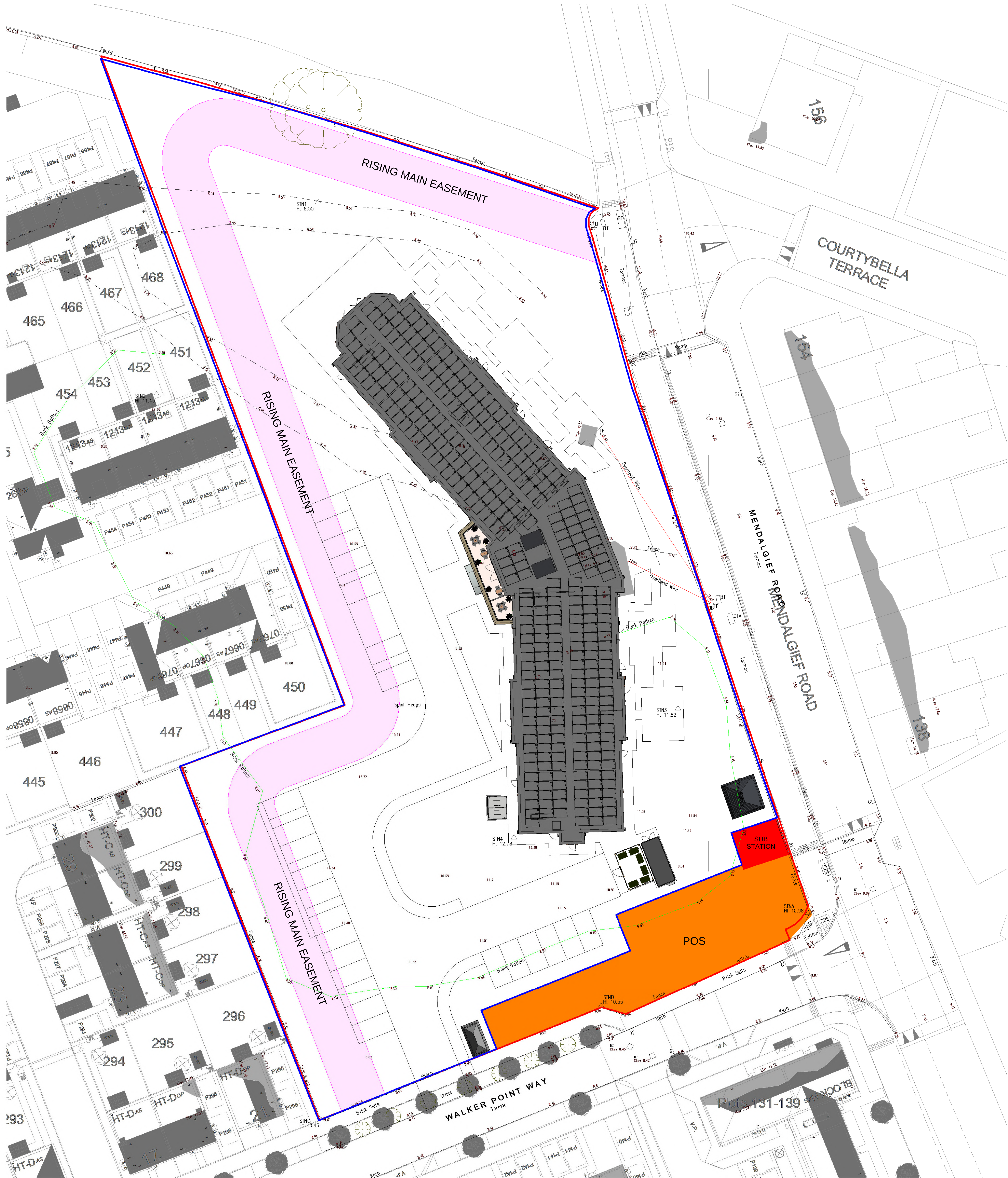
CONSTRAINTS OVERLAY 1 : 200
