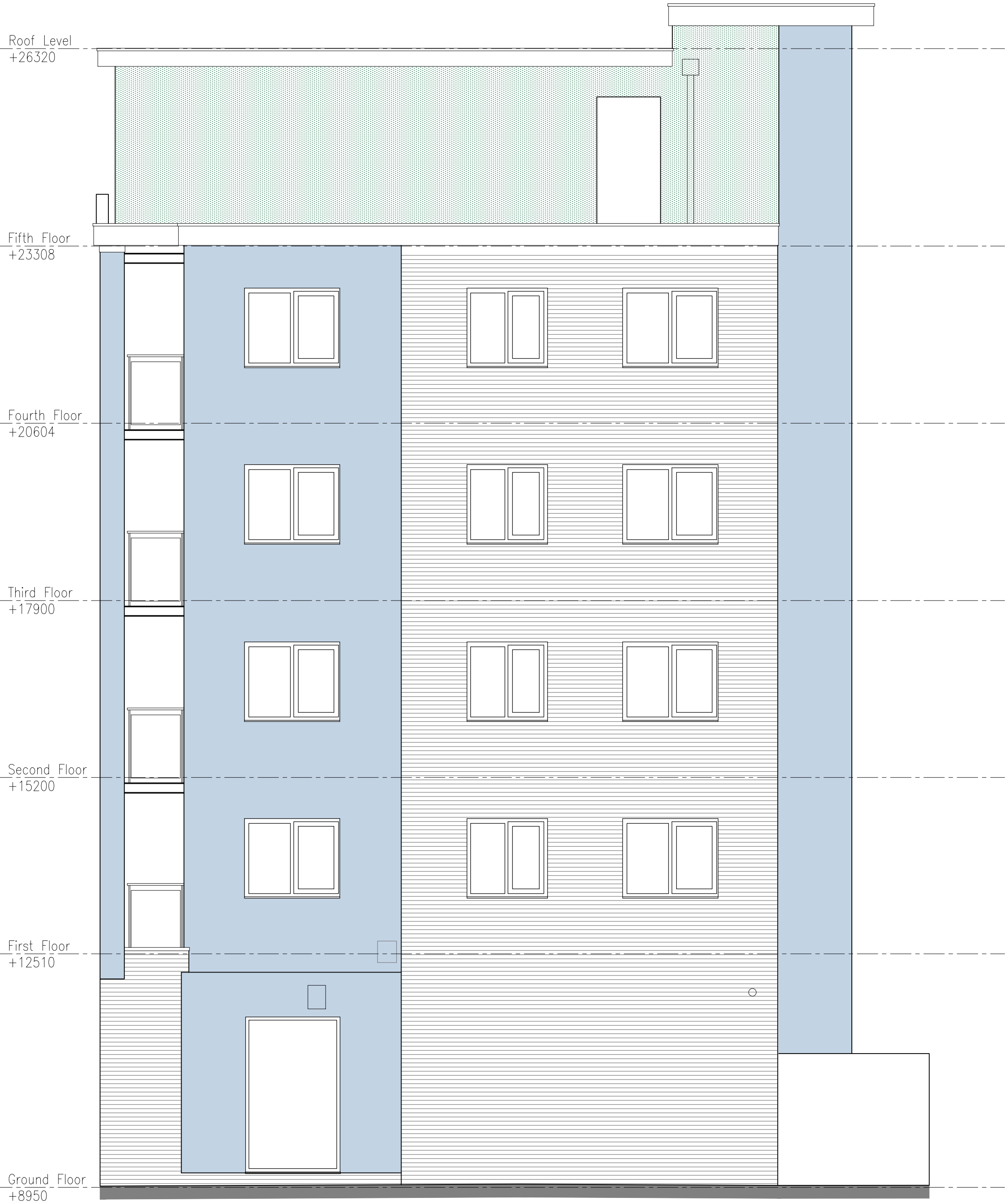
Elevation 3.
