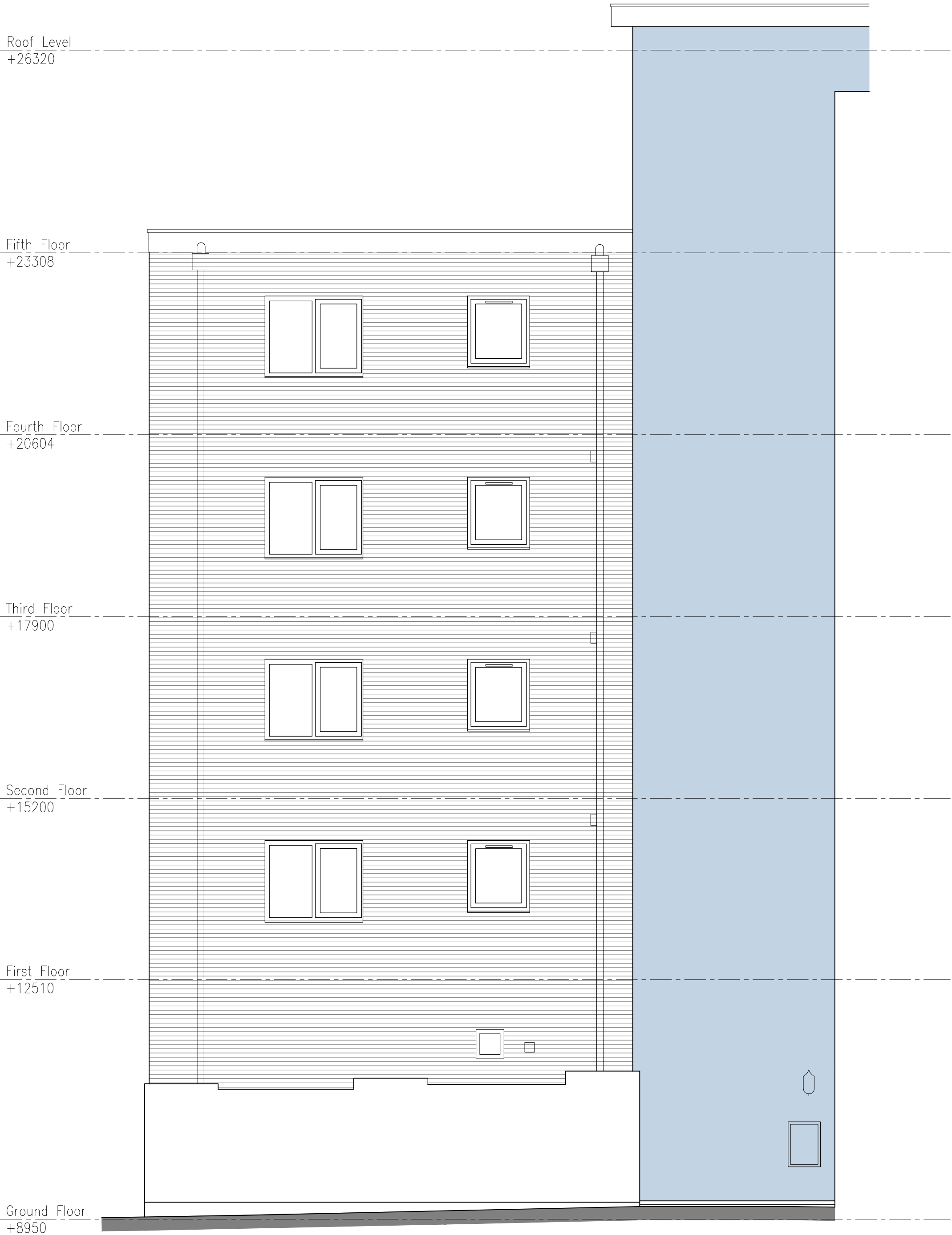
Elevation 4.
