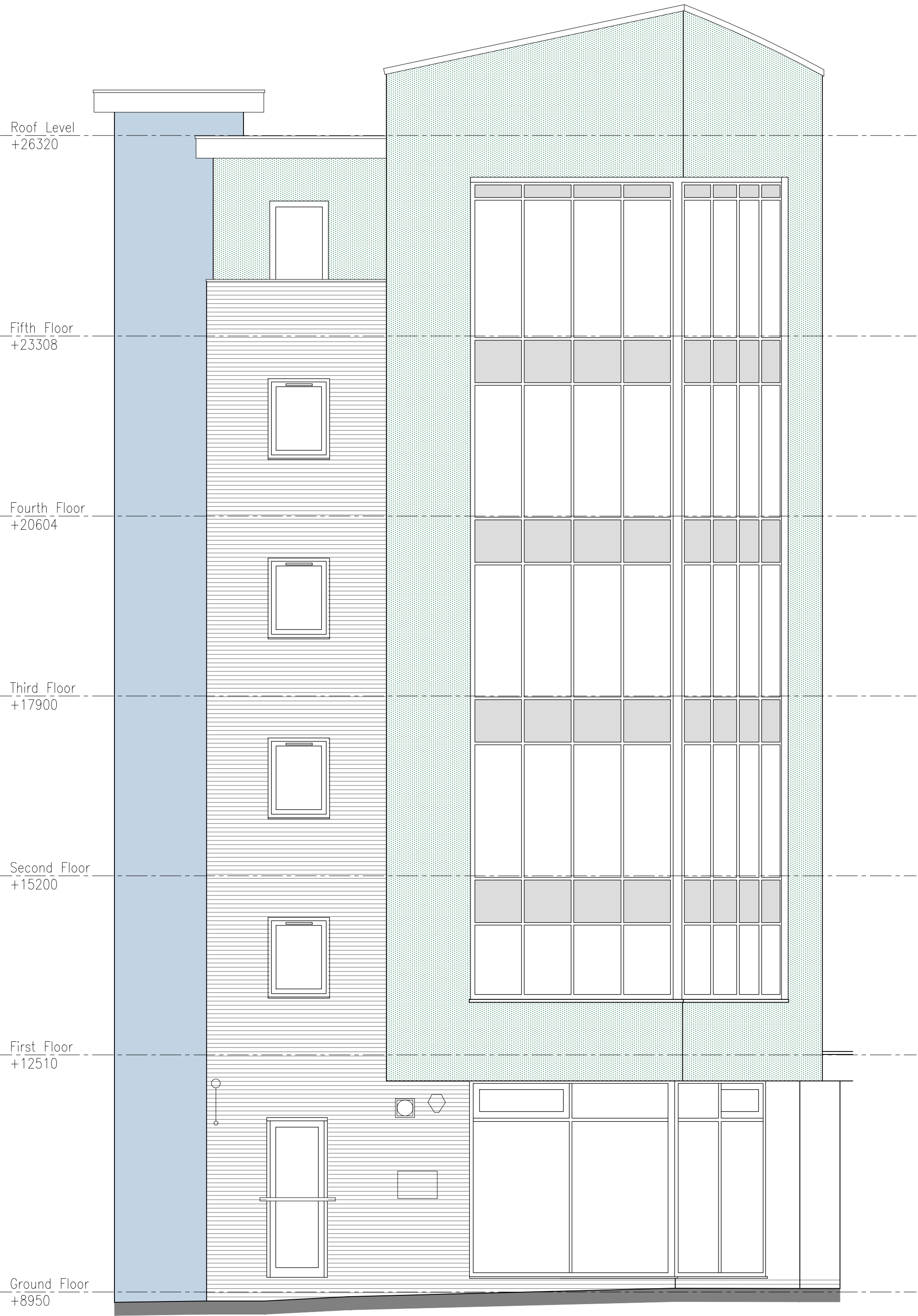
Elevation 6.
