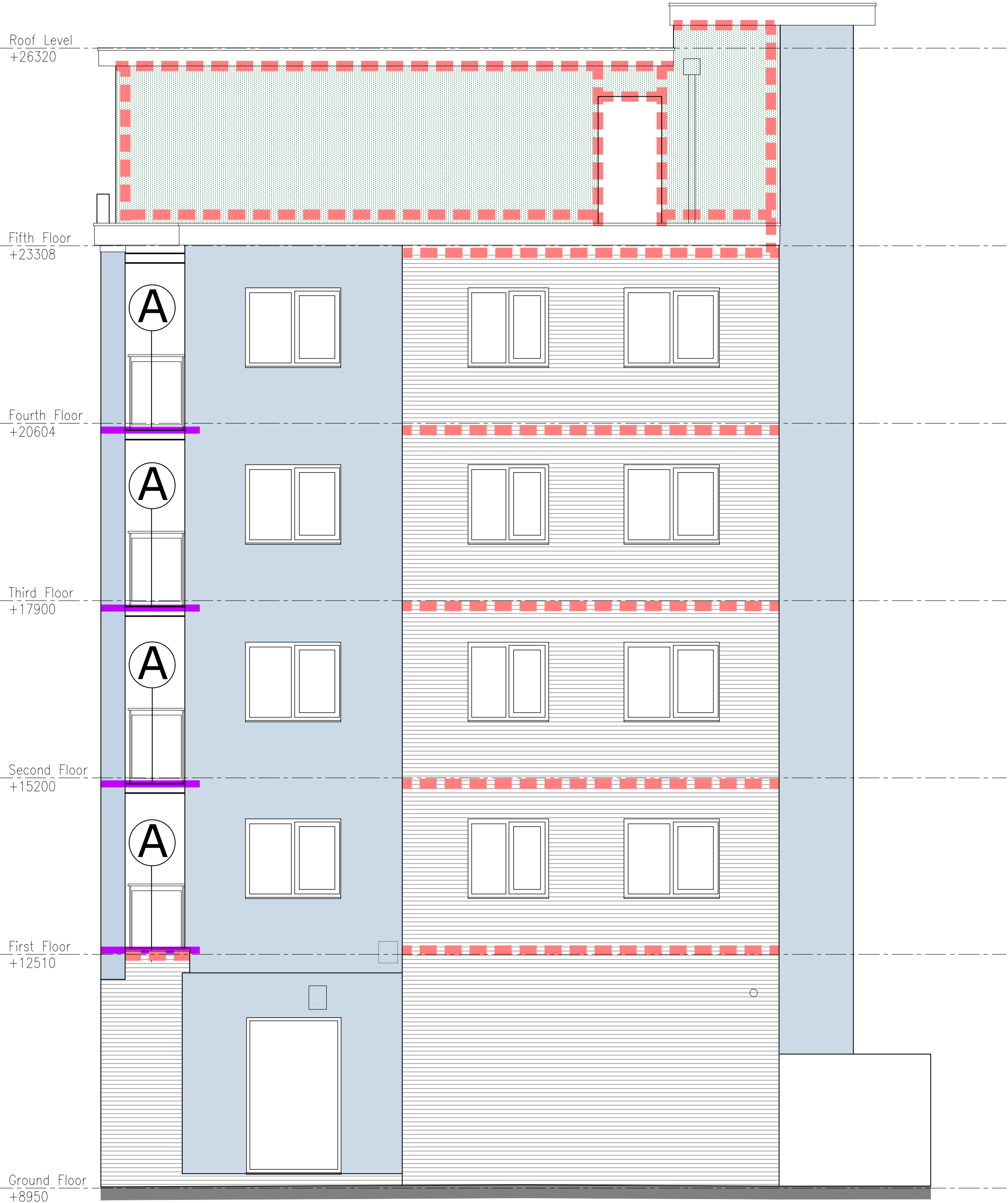
Elevation 3.
