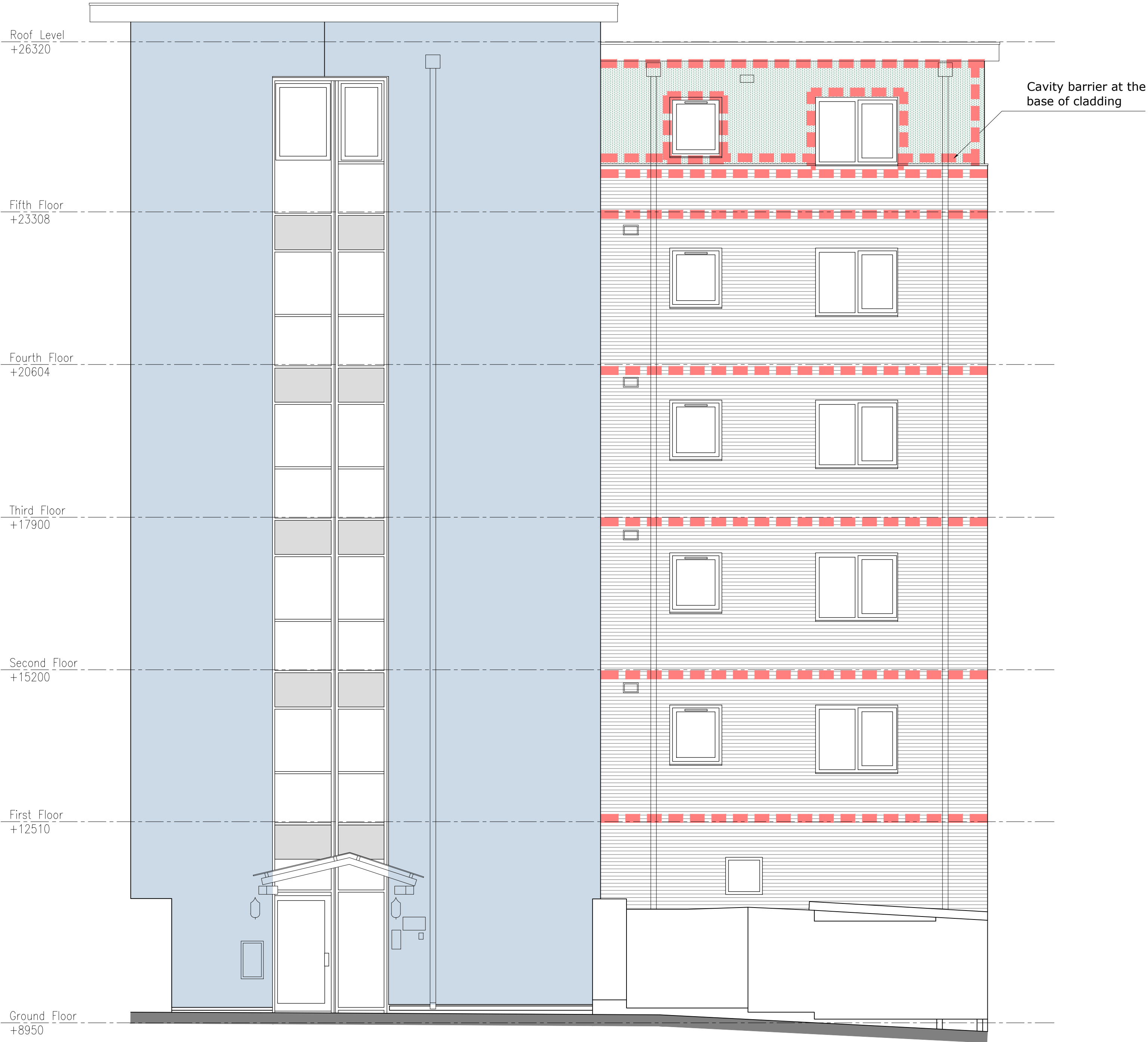
Elevation 5.
