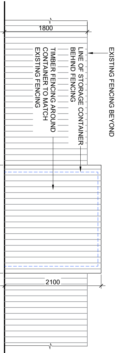
SIDE ELEVATION 2 AS PROPOSED
