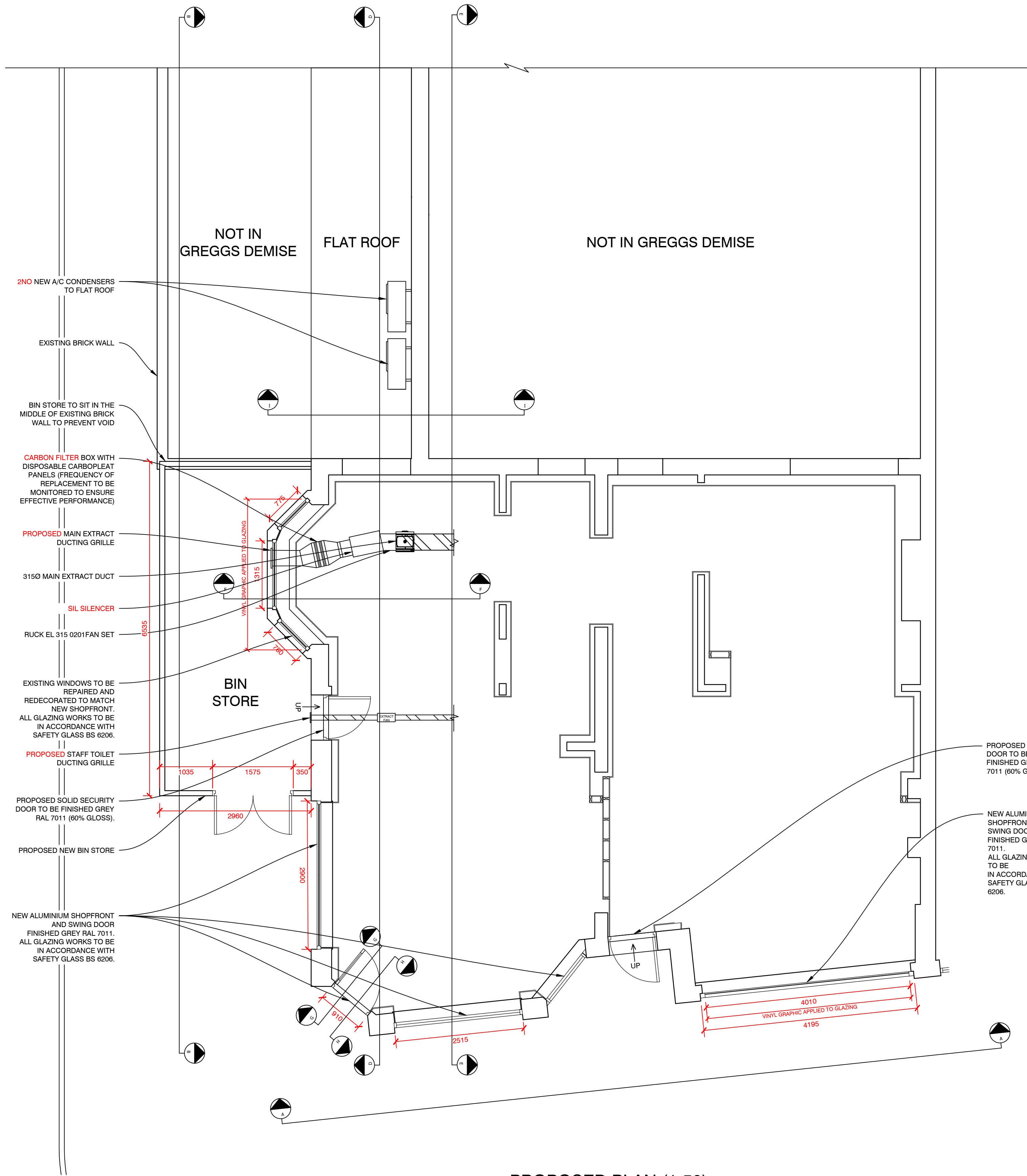
PROPOSED PLAN (1:50)
