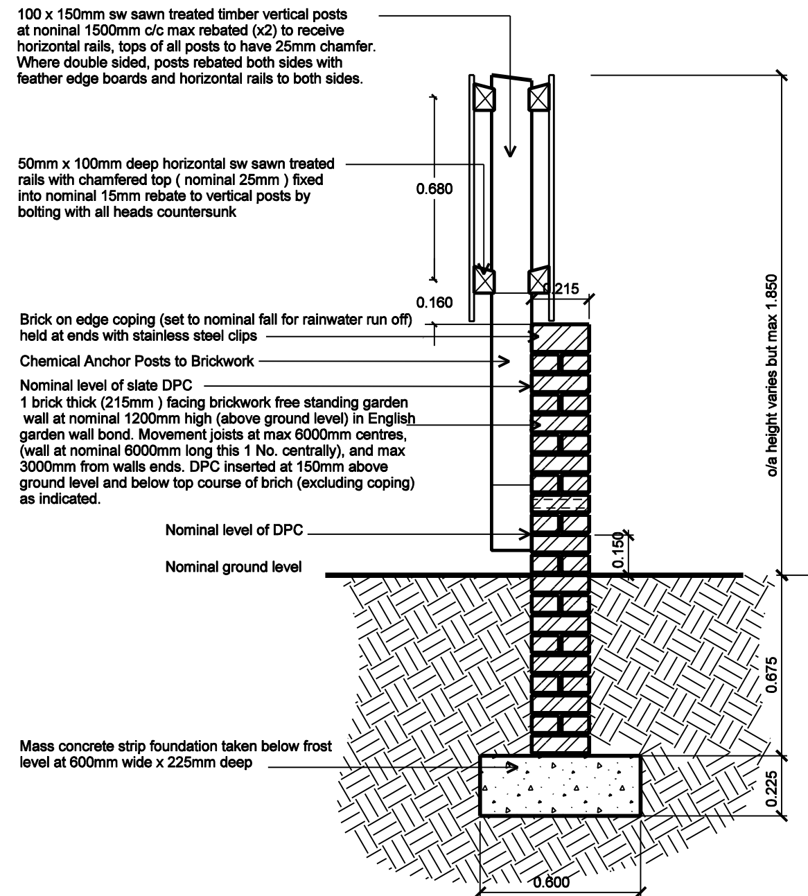
Free Standing Boundary Wall
