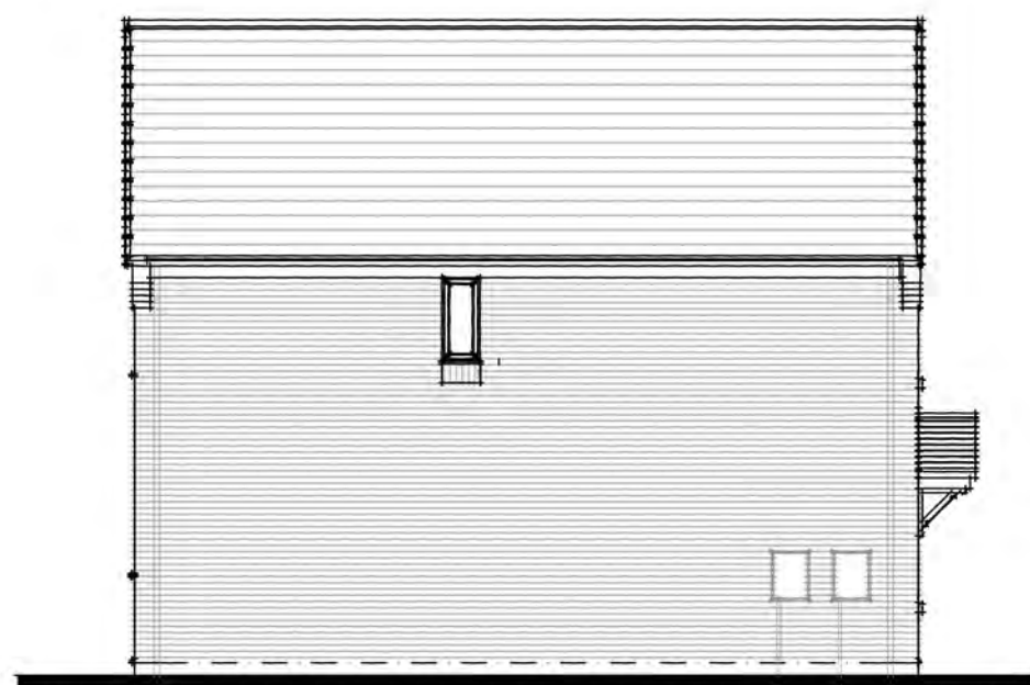
SIDE B ELEVATION
