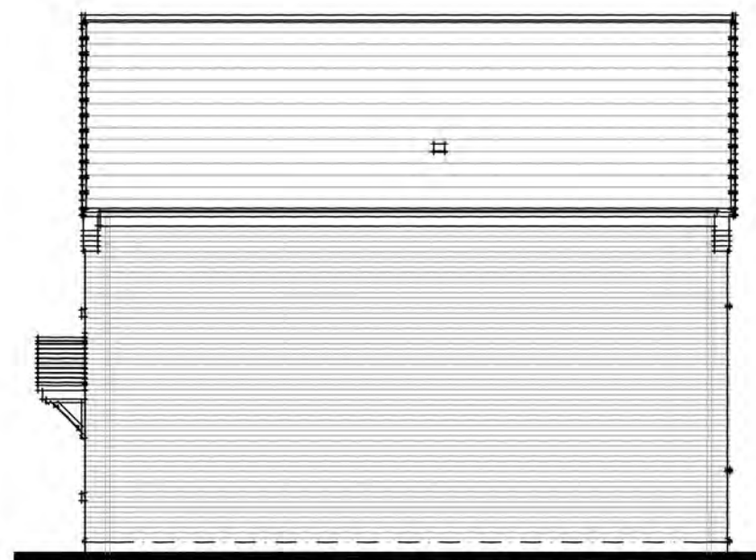
SIDE A ELEVATION
