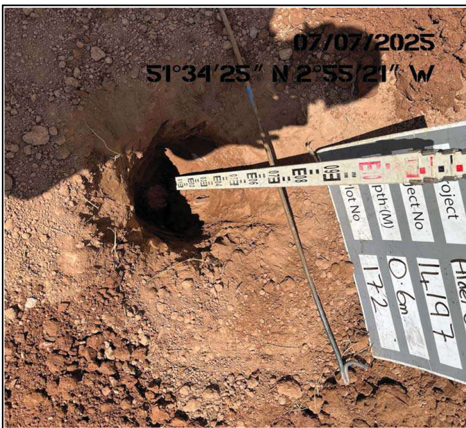
Plot 172 Trial Pit Excavation Profile
