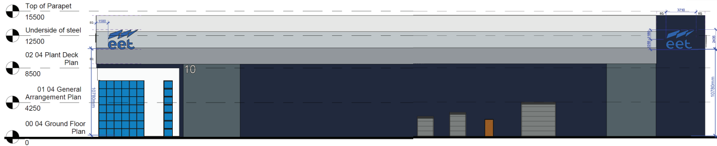
1 West Face Elevation
