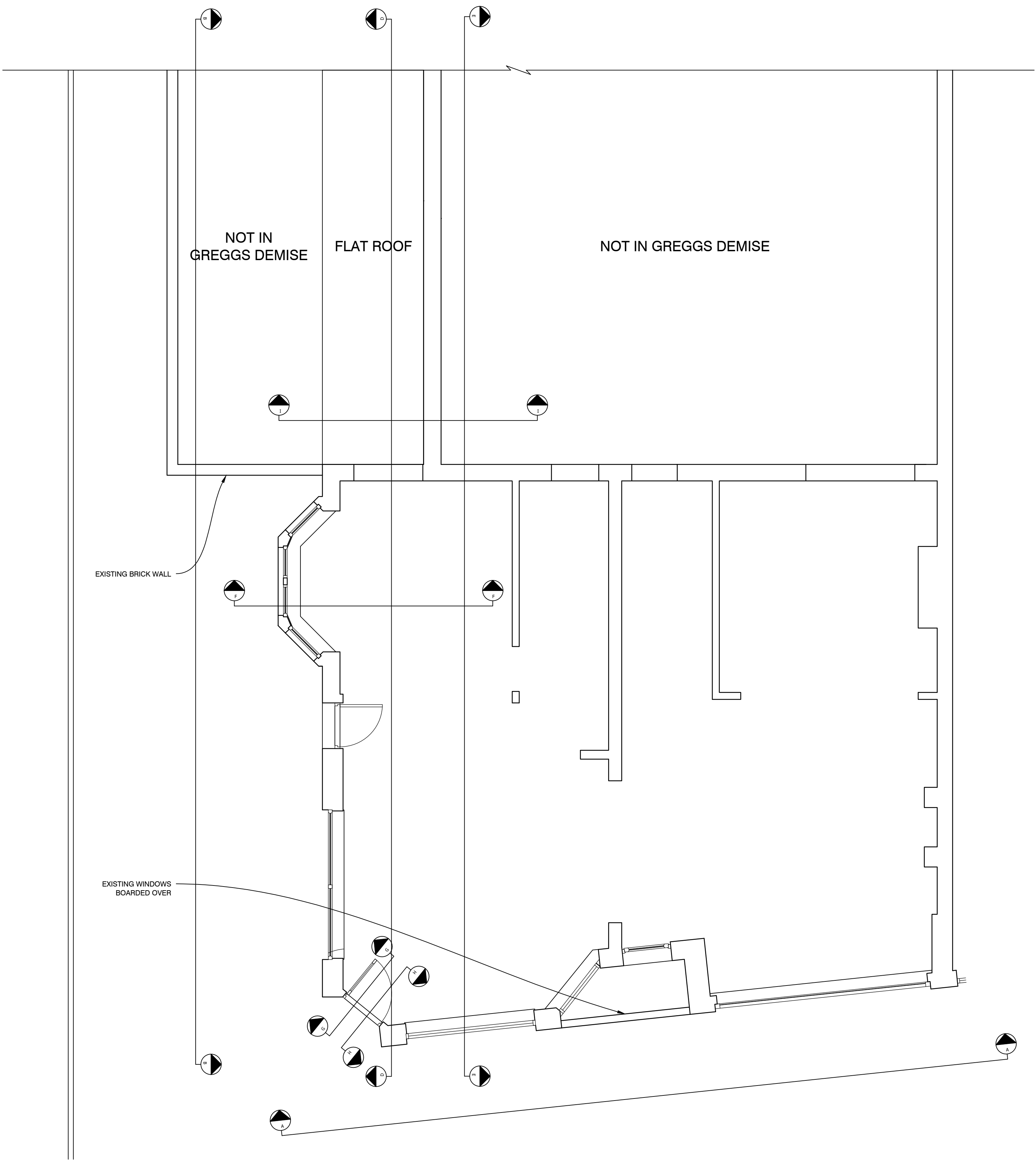
EXISTING PLAN (1:50)
