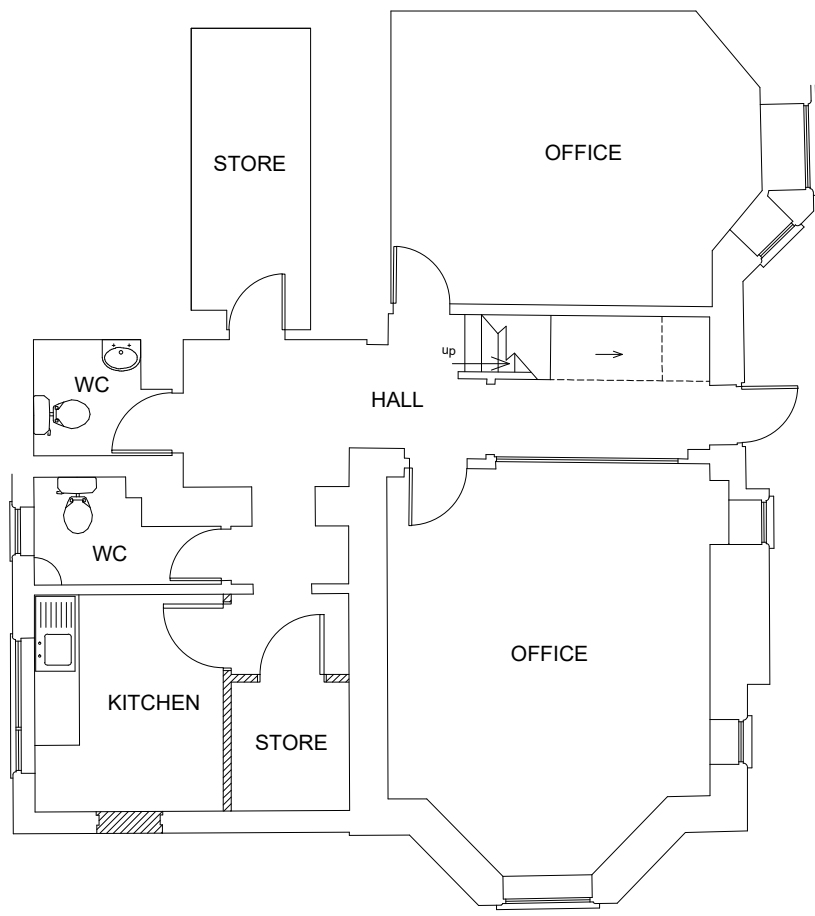
Basement Plan
