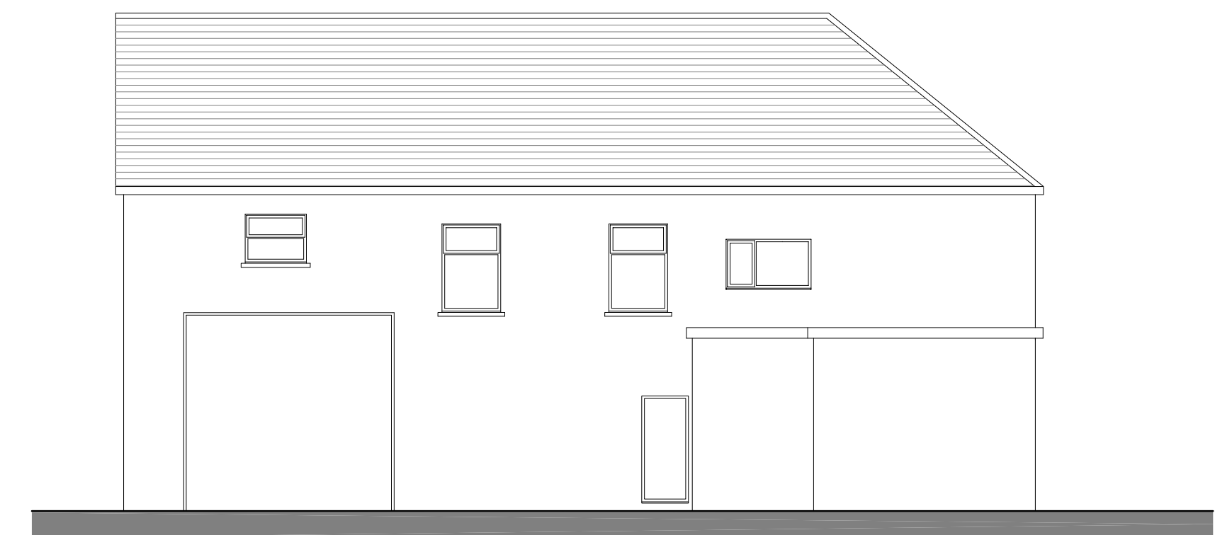
REAR ELEVATION
