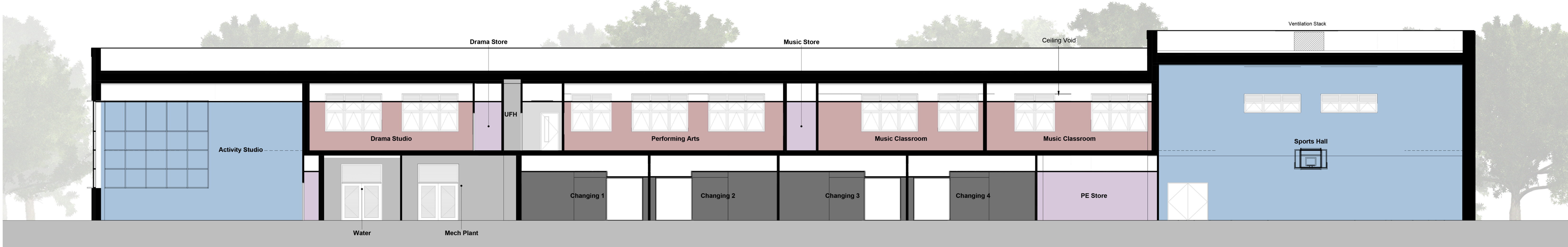
Section X3 Coloured Scale: 1 : 100
