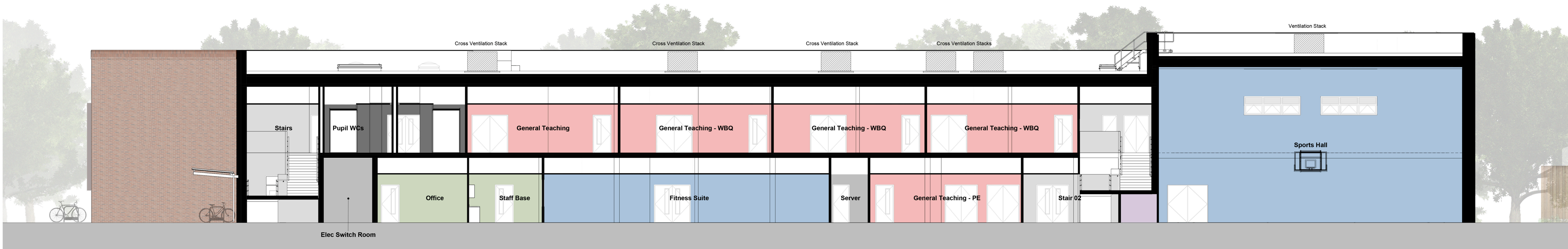
Section X1 Coloured Scale: 1 : 100
