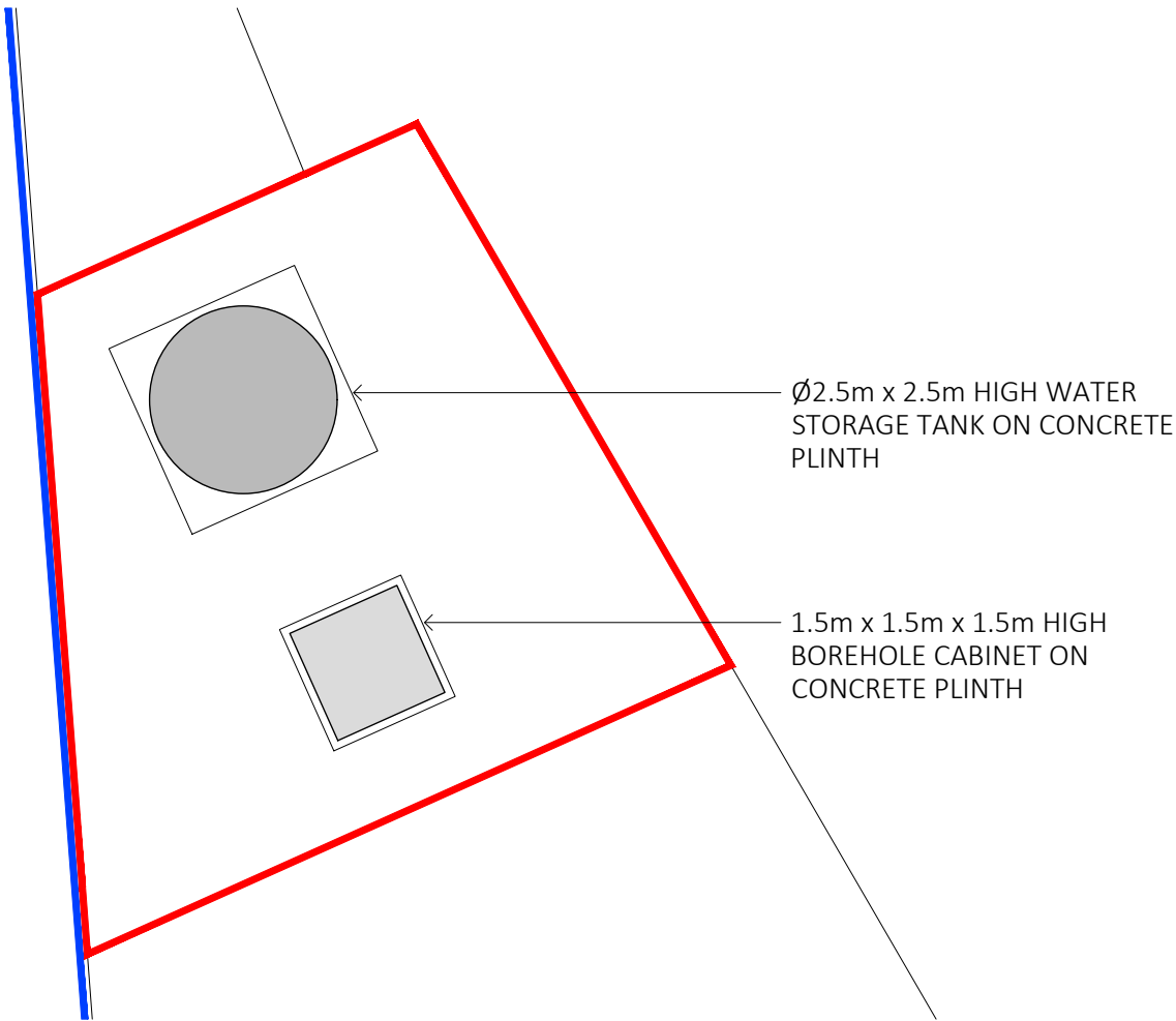
SITE PLAN (1:100)
