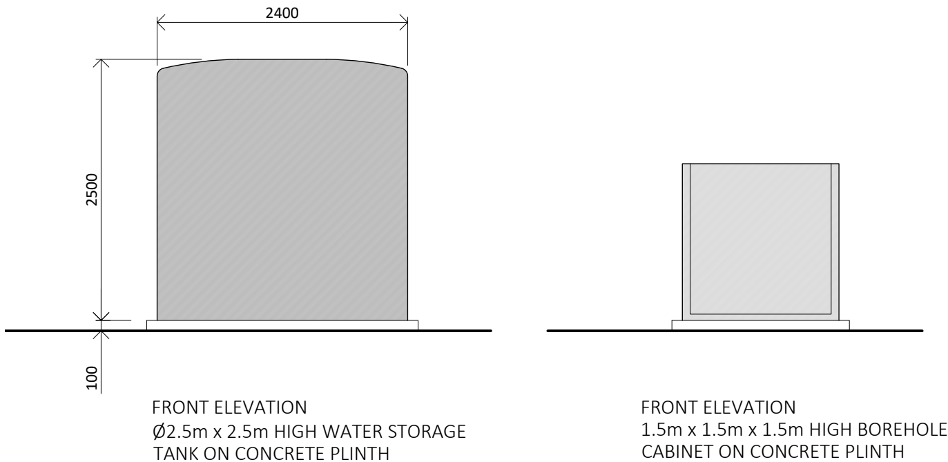
WATER STORAGE TANK AND BOREHOLE CABINET DETAILS (1:50)
