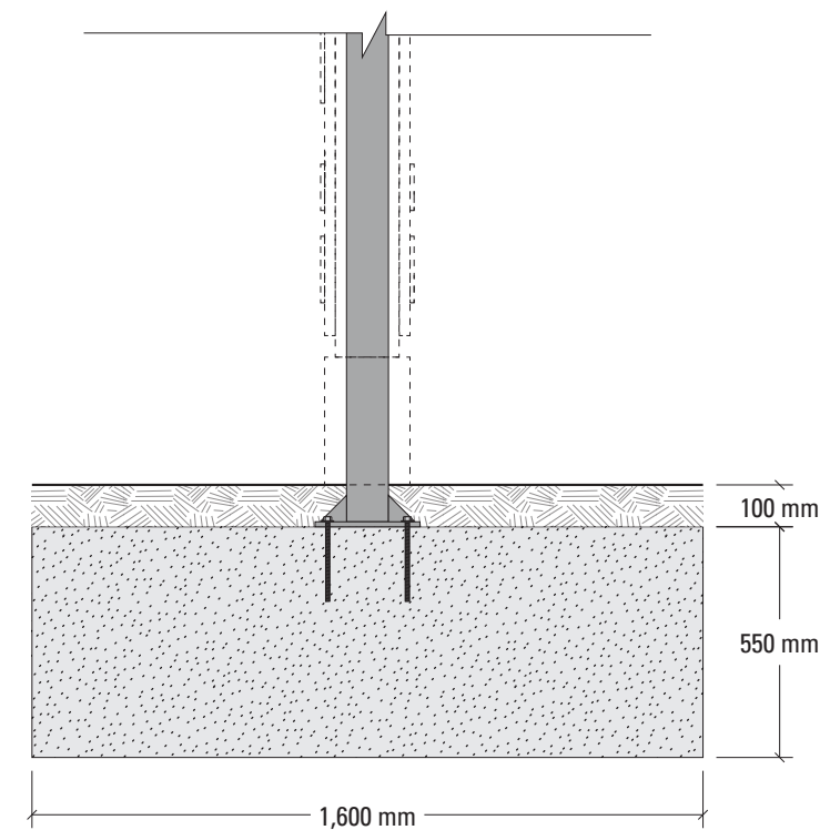
TYP. FOOTING DETAIL - SIDE VIEW Scale: 1:20
