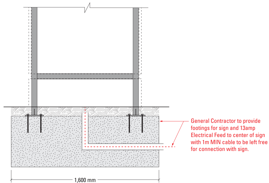
TYP. FOOTING DETAIL - FRONT VIEW Scale: 1:20
