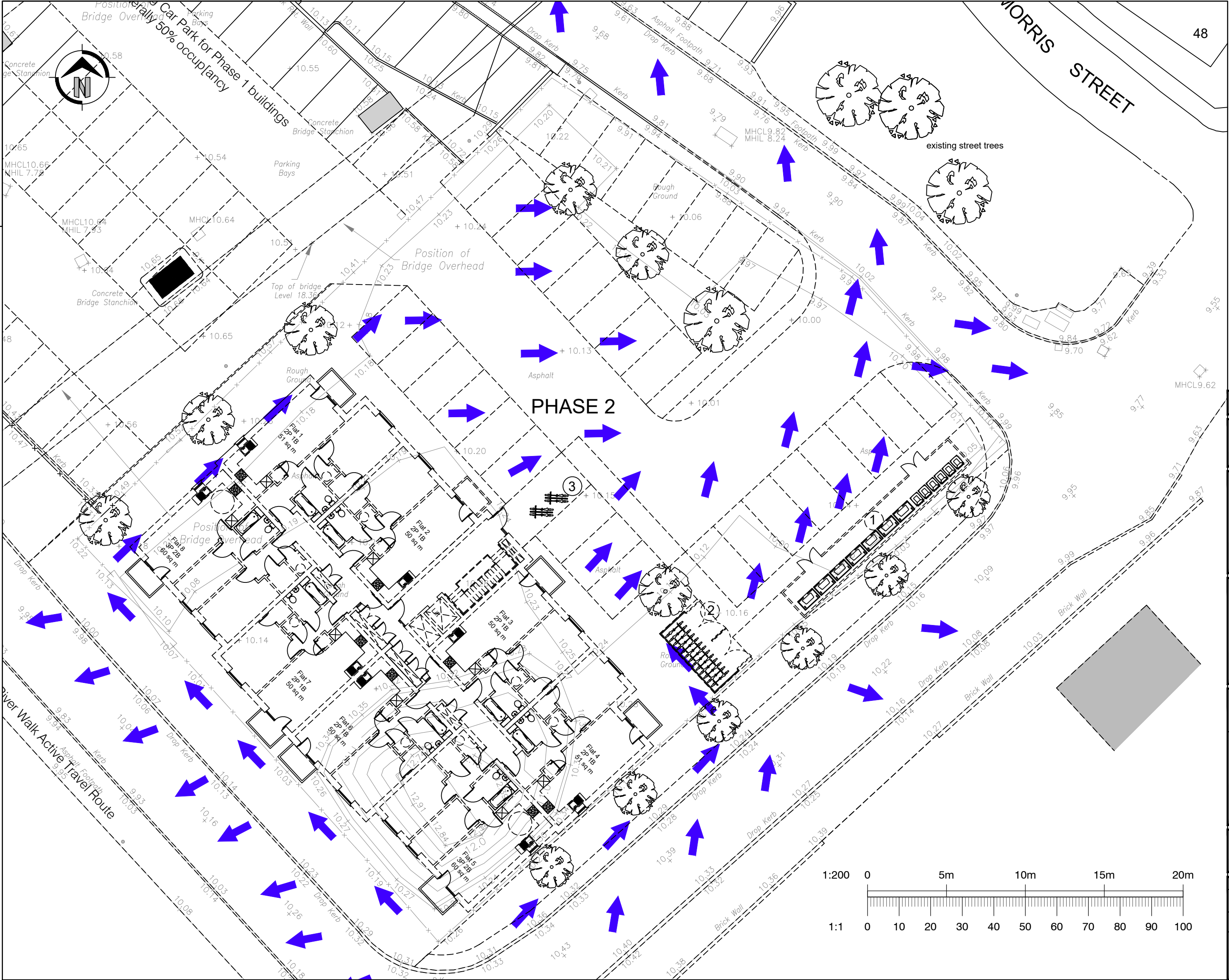
Proposed Overland Flow Path 1:200
