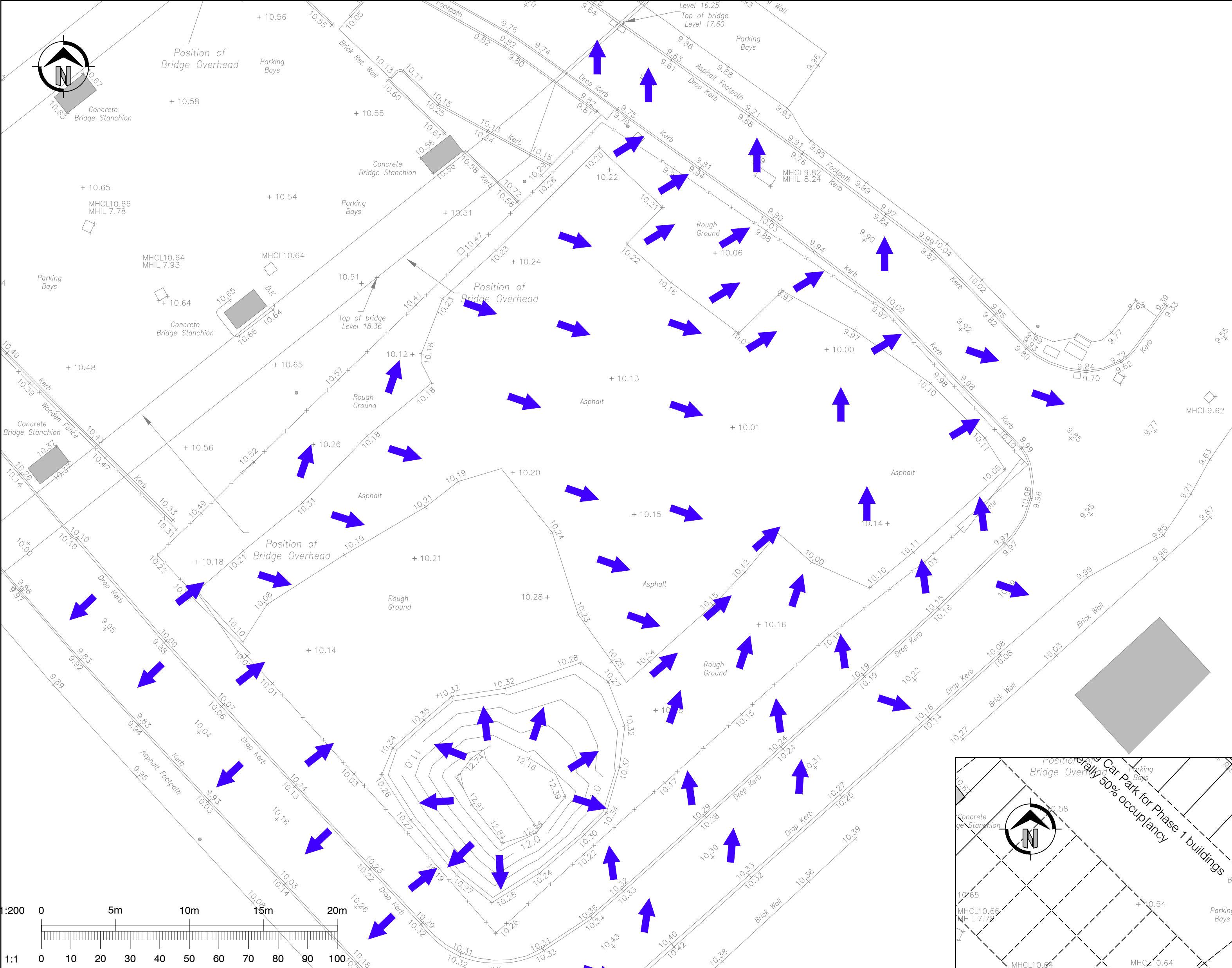
Existing Overland Flow Path 1:200
