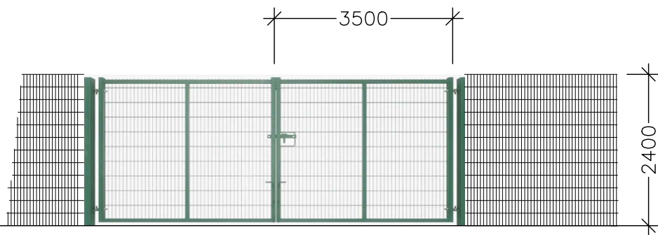
SECURITY GATES-Colour to match fence
