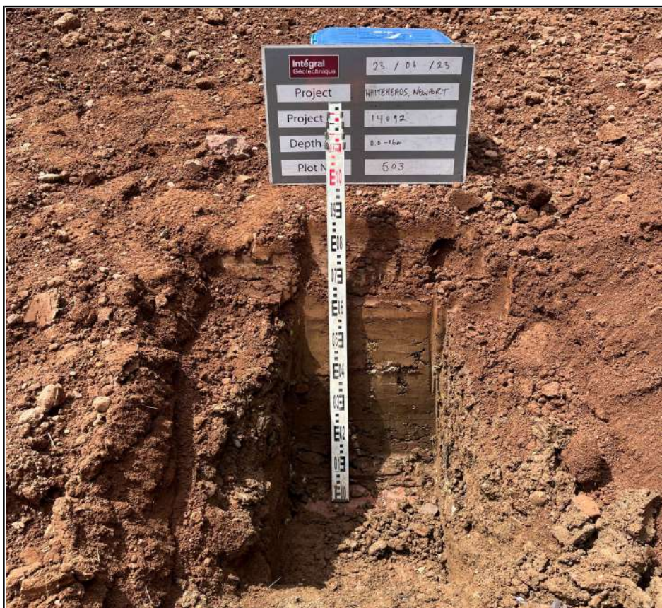
Plot 311 Trial Pit Excavation and Membrane Check
