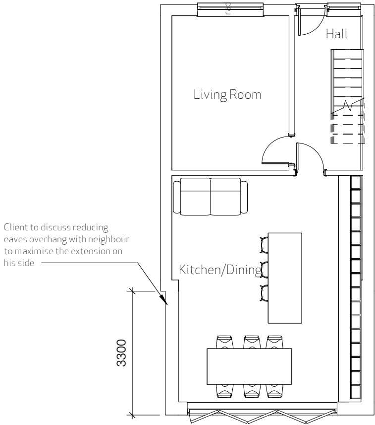
1 Ground Floor as Proposed 1:100
