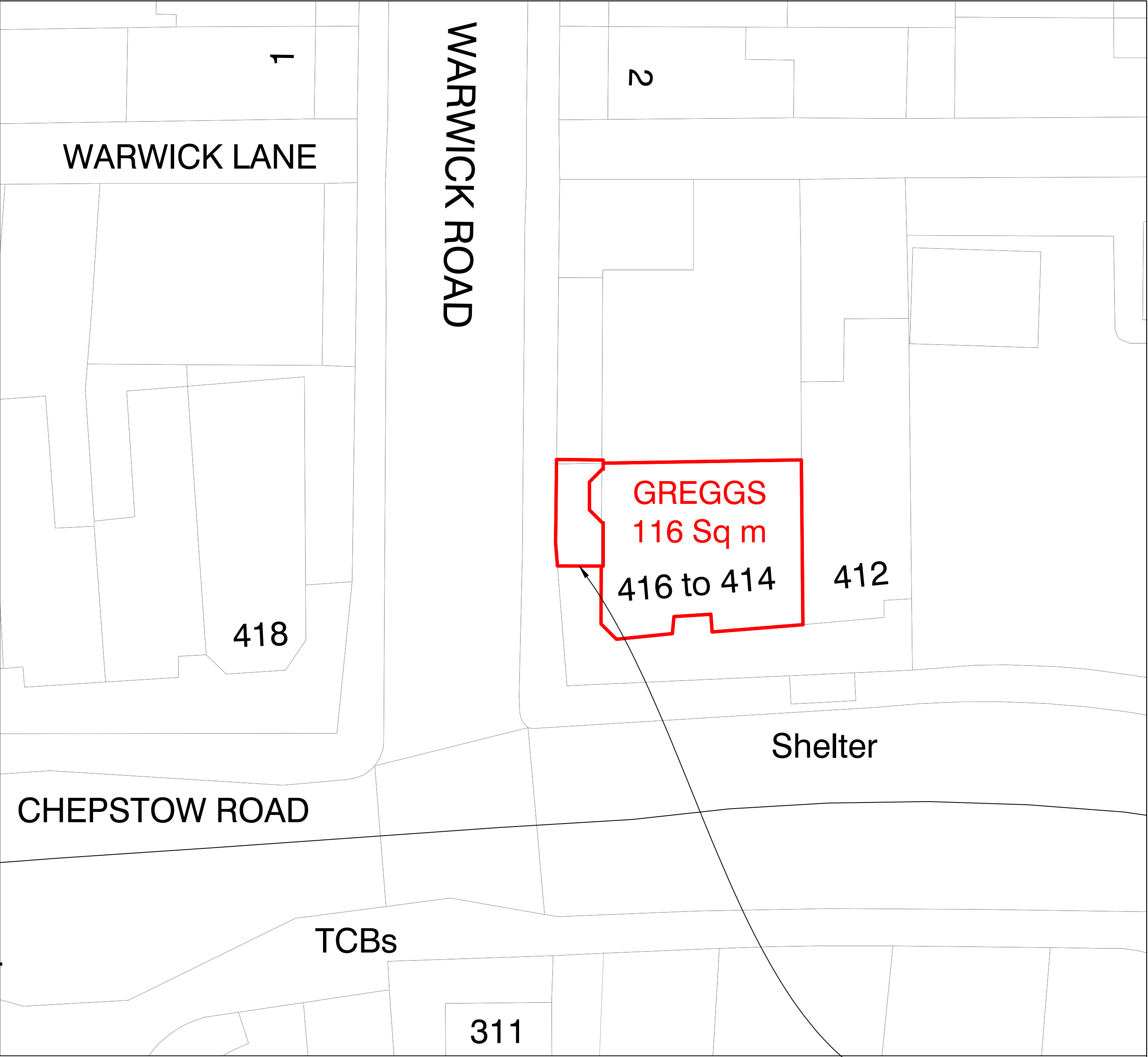
PROPOSED BLOCK PLAN (1:200) SCALE 1:200
