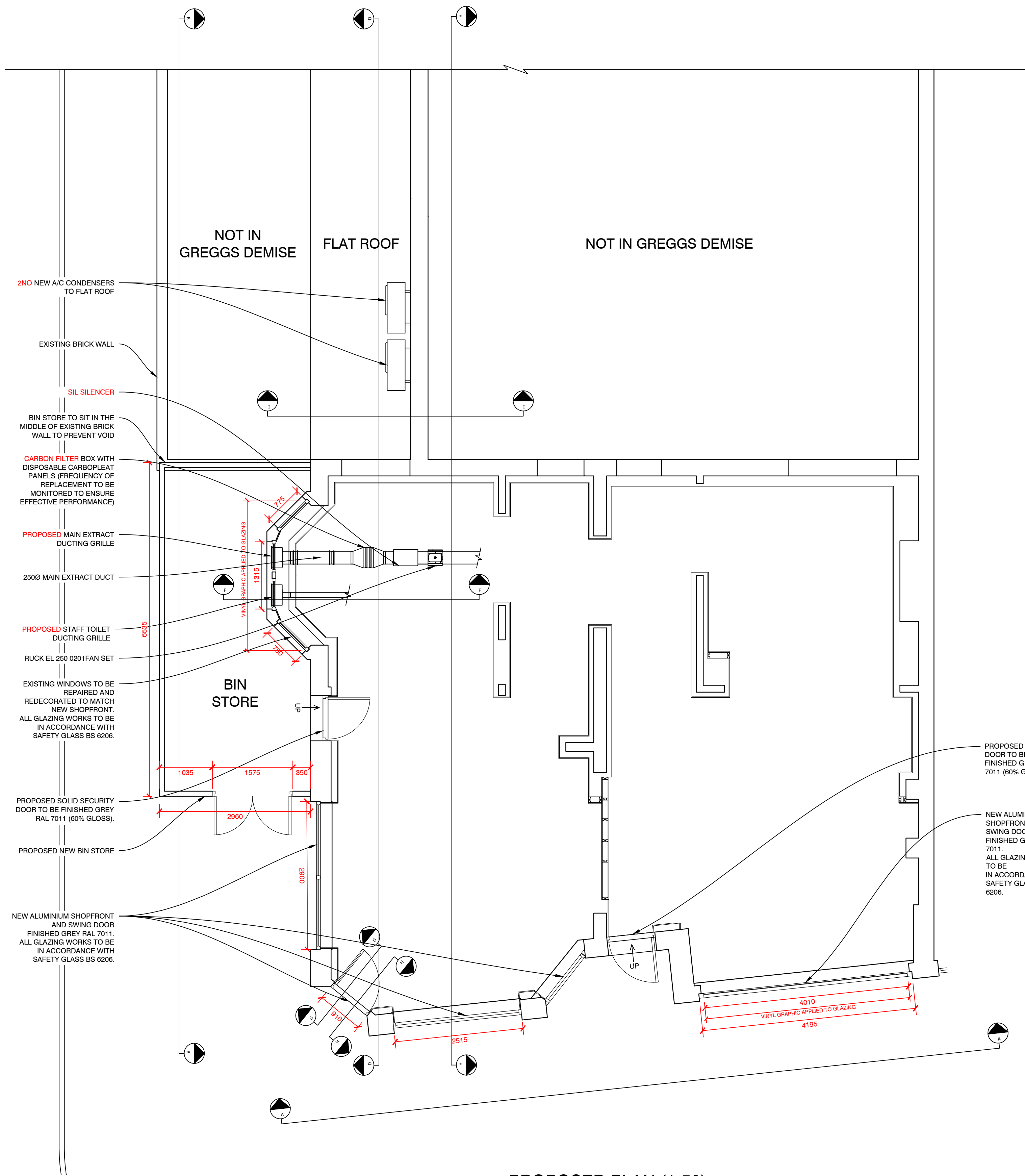
PROPOSED PLAN (1:50)
