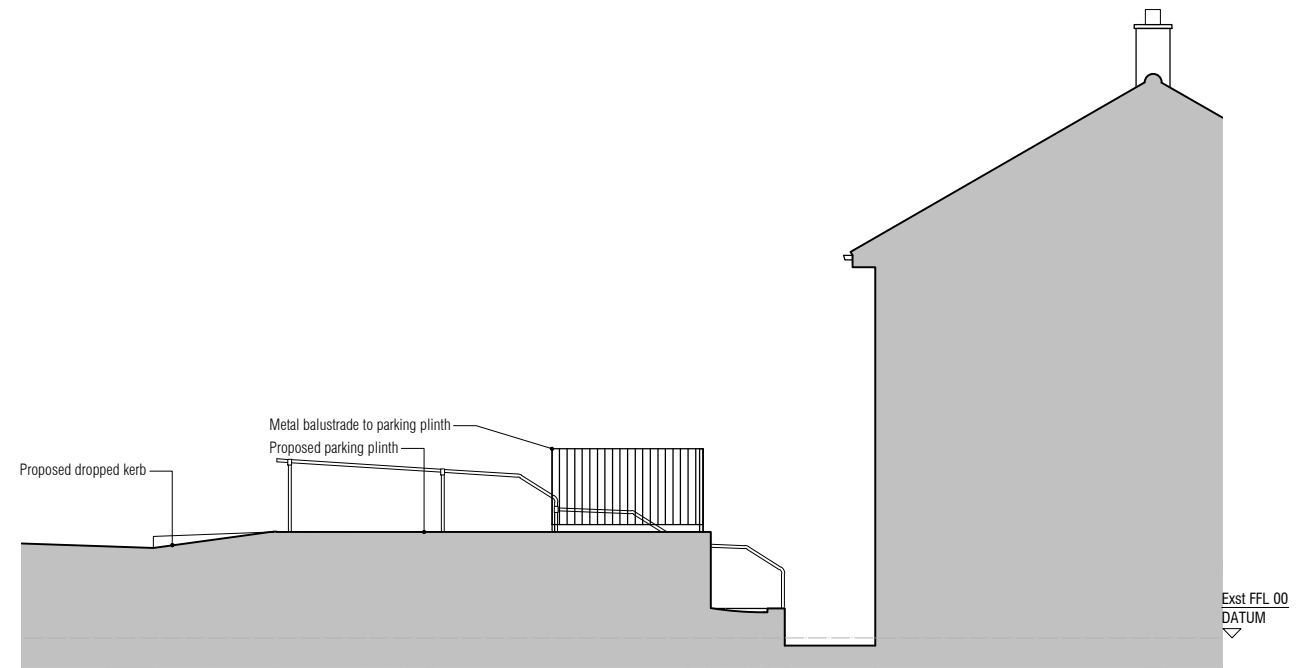
2. PROPOSED SECTION
