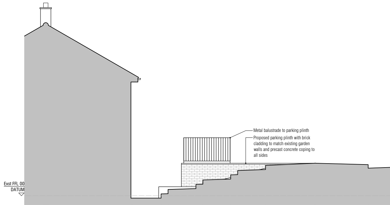
1. PROPOSED SECTION
