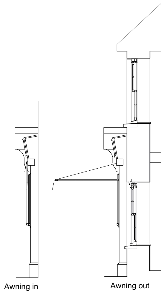
Section through W02/W11, as Proposed; 1:50
