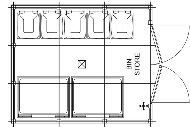
FLOOR PLAN
