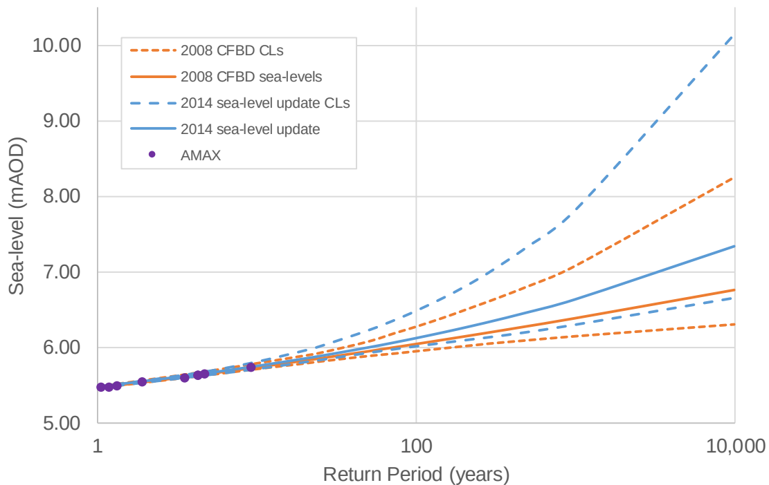
Figure A. 11-7: Mumbles 2008 and 2014 sea-level return periods
