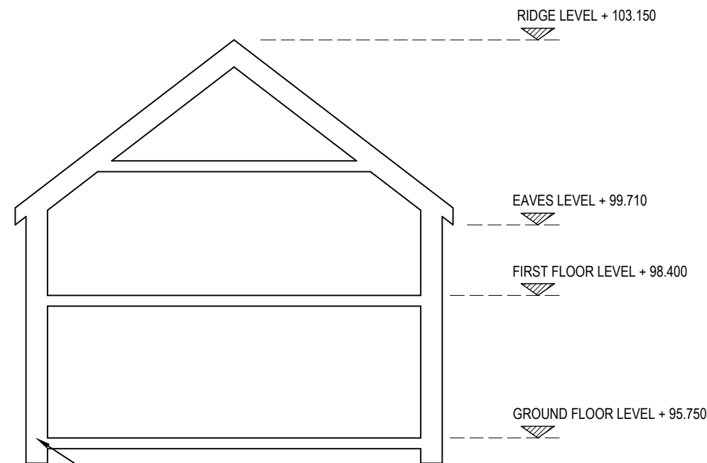
TYPICAL SECTION
