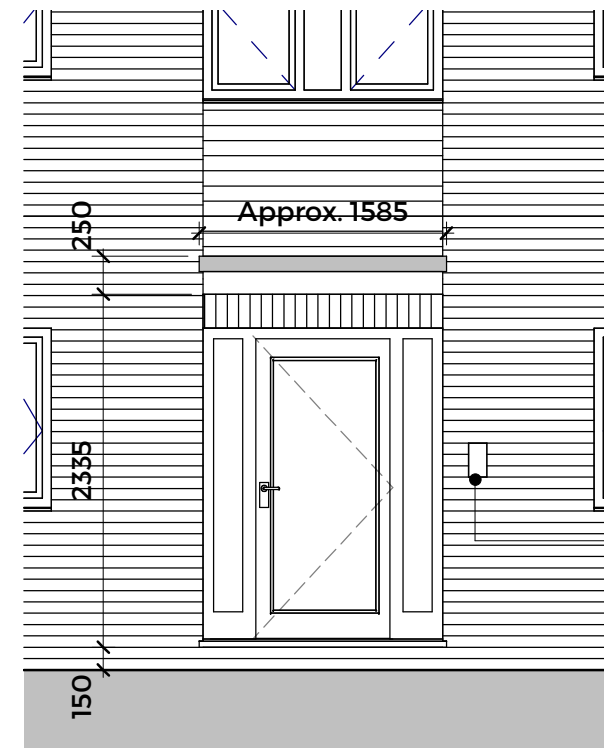
Canopy Elevation 1 : 50
