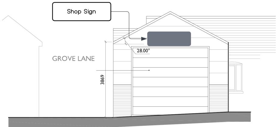
CLYTHA SQUARE ELEVATION - (NORTH EAST ELEVATION)
