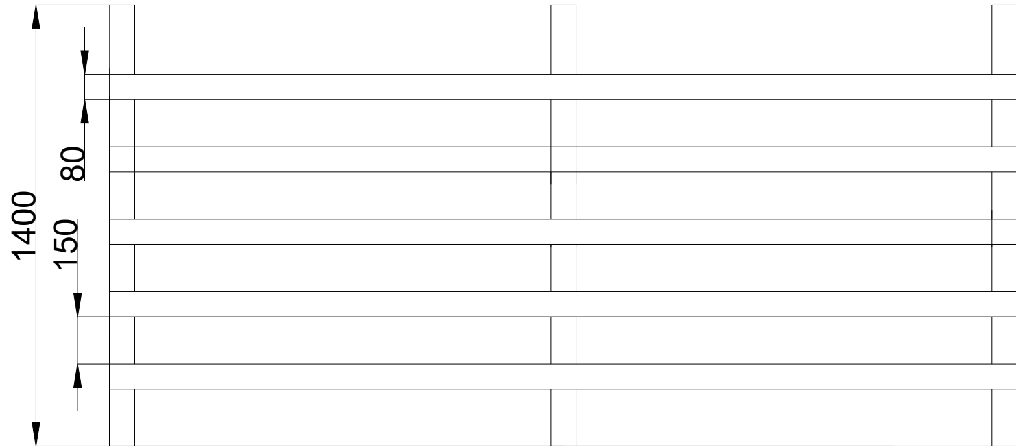
1.4m RANCH RAIL
