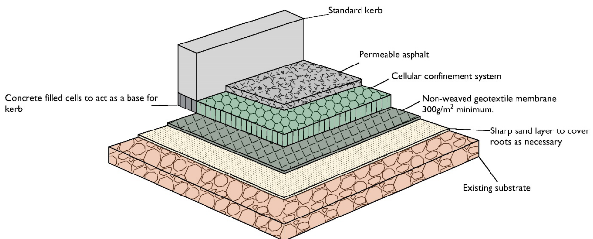
Figure 1b. a conceptual diagram outlining the design principle. (ASPHALT ROAD)
