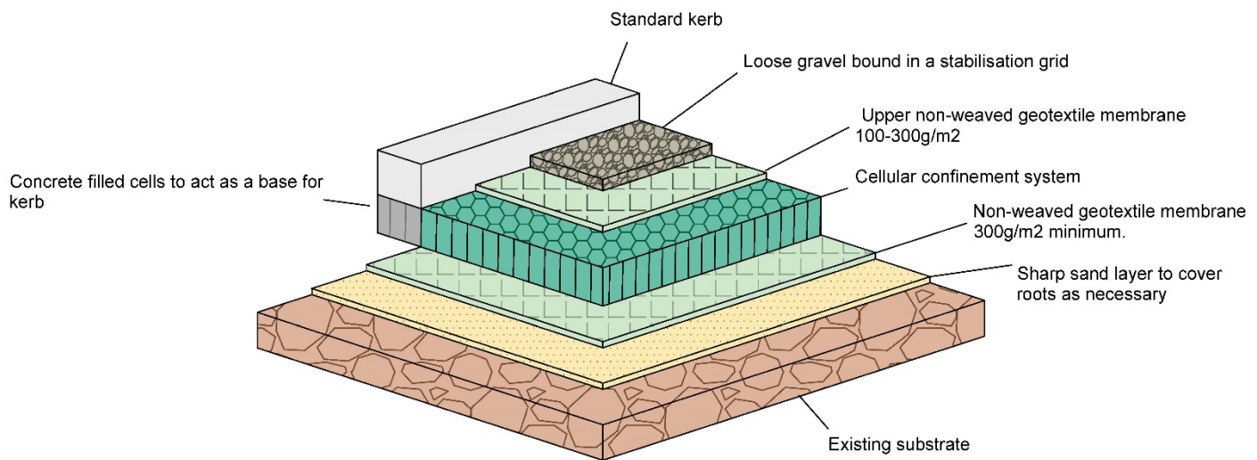
Figure 1a. a conceptual diagram outlining the design principle. (GRAVEL ROAD)
