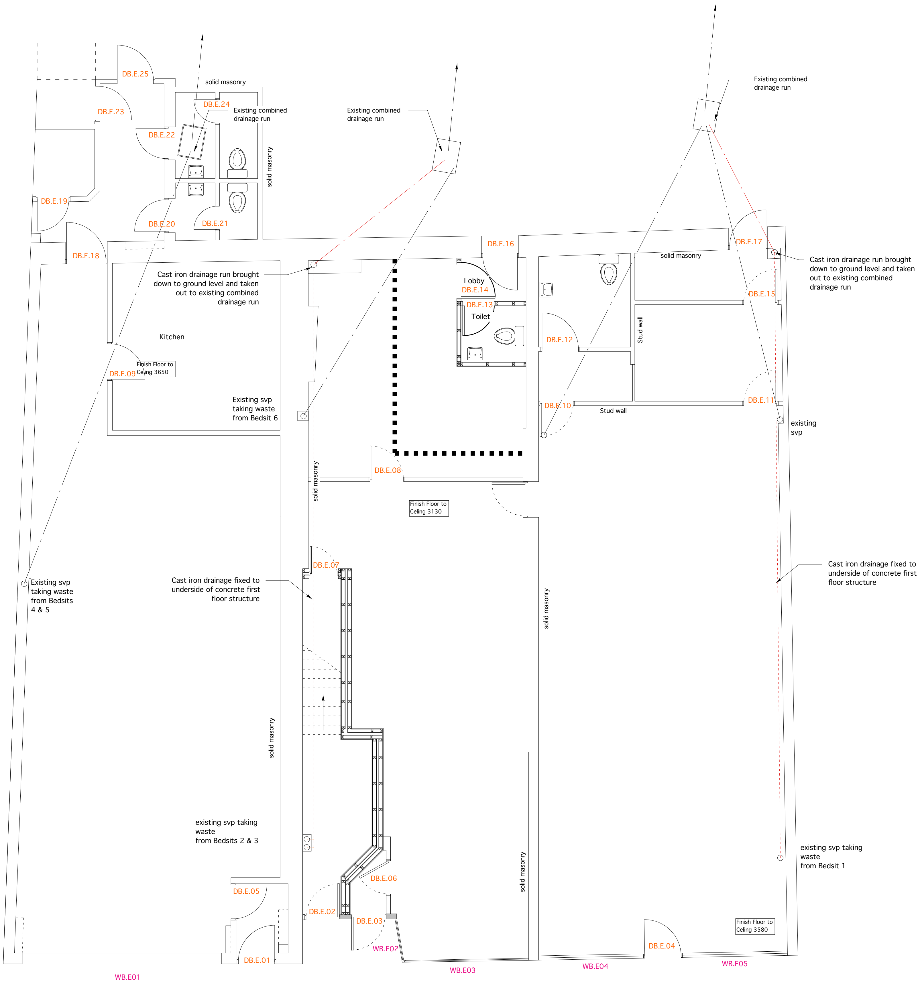
GROUND FLOOR
